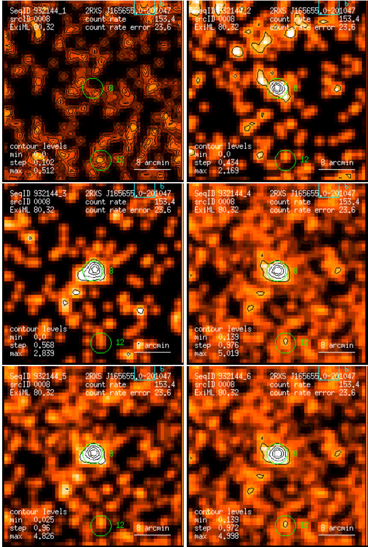
Figure 8: RASS 932144: detection 0008: band rate images, Gaussian filter: (1) PSPC channels 11 – 41, (2) 52 – 90, (3) 91 – 201, (4) 11 – 235, (5) 52 – 201, (6) 11 – 201. Broad band rates in counts/ks. Band rate contour levels in counts/ks/arcmin 2 .
