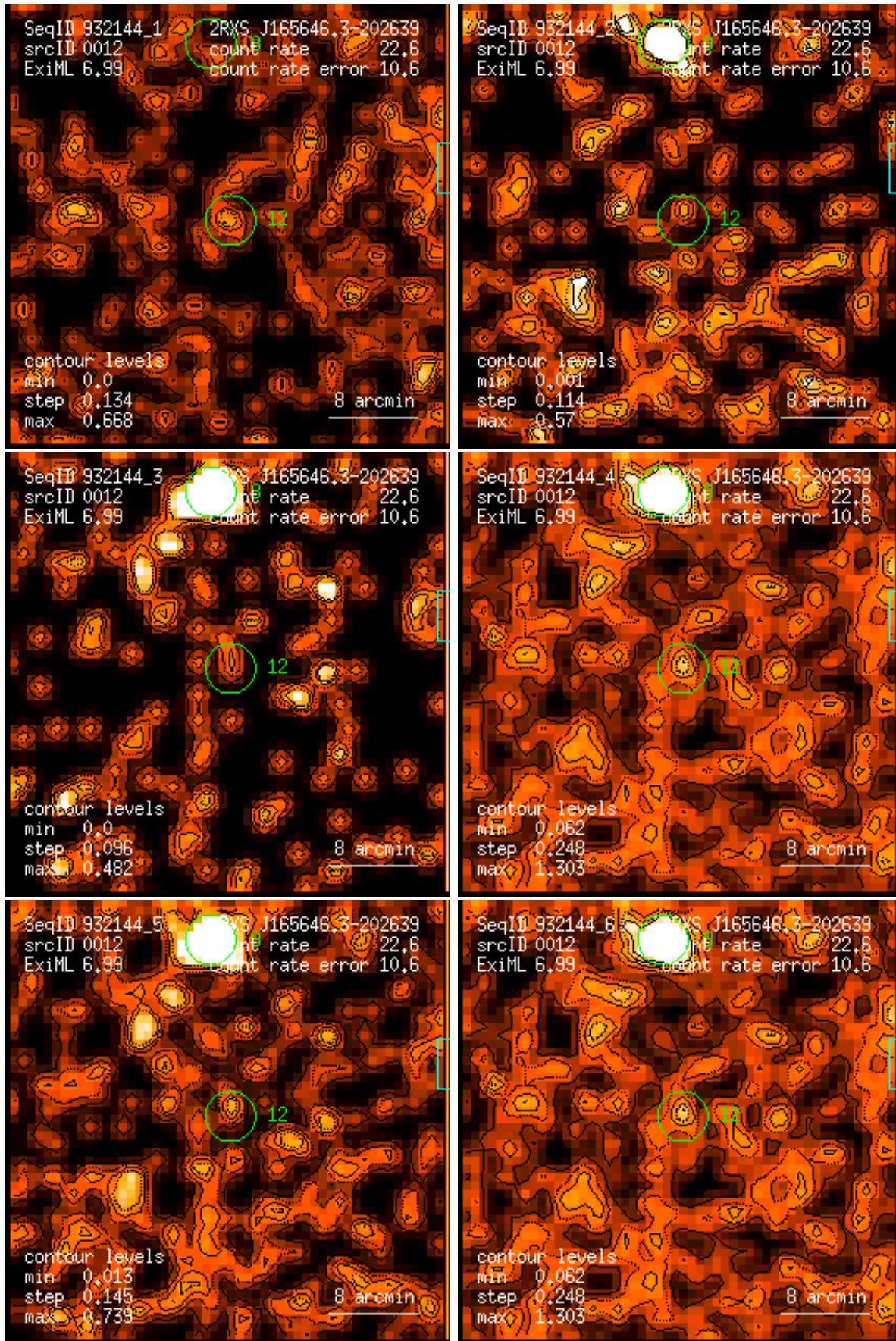
Figure 12: RASS 932144: detection 0012: band rate images, Gaussian filter: (1) PSPC channels 11 – 41, (2) 52 – 90, (3) 91 – 201, (4) 11 – 235, (5) 52 – 201, (6) 11 – 201. Broad band rates in counts/ks. Band rate contour levels in counts/ks/arcmin 2 .
