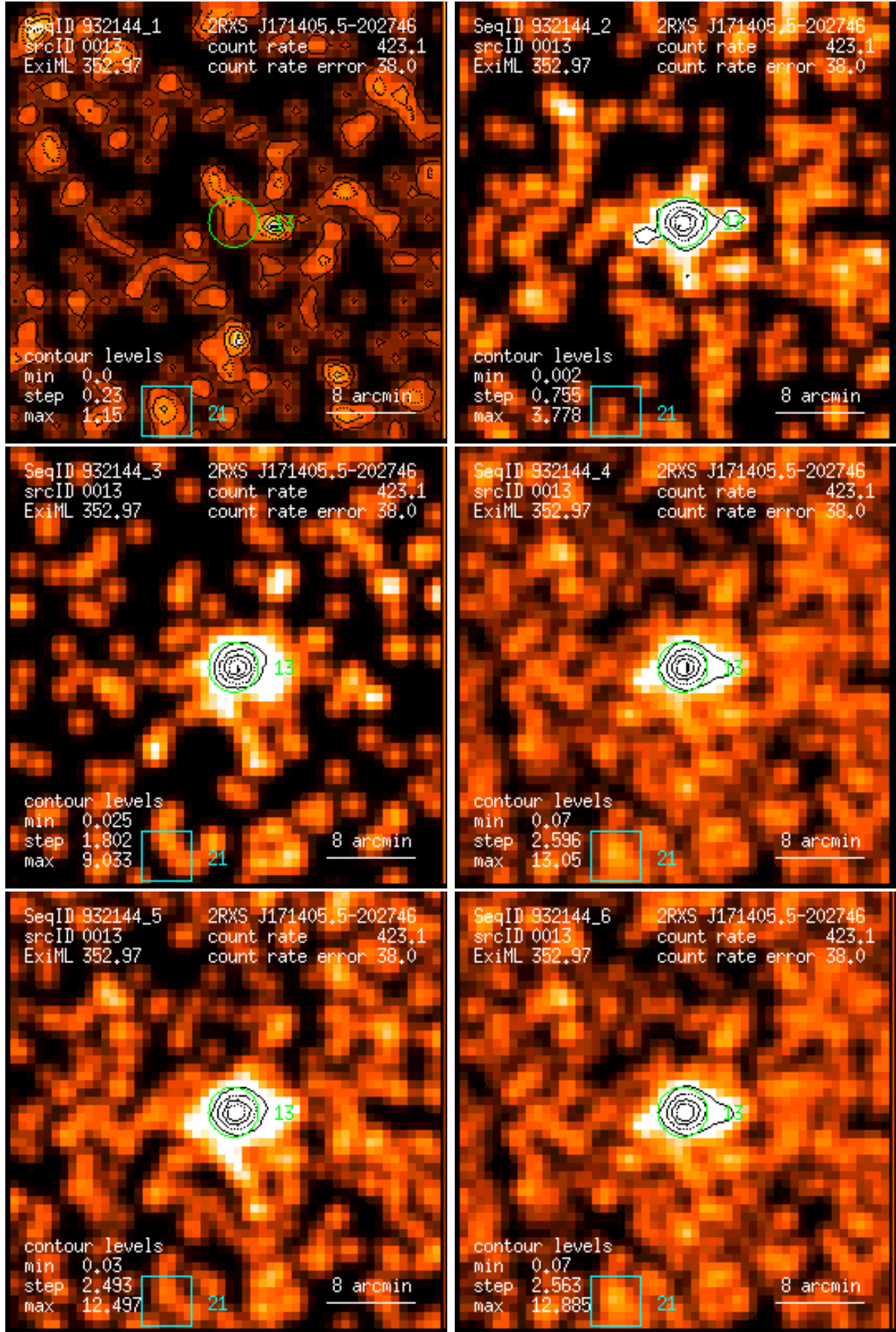
Figure 13: RASS 932144: detection 0013: band rate images, Gaussian filter: (1) PSPC channels 11 – 41, (2) 52 – 90, (3) 91 – 201, (4) 11 – 235, (5) 52 – 201, (6) 11 – 201. Broad band rates in counts/ks. Band rate contour levels in counts/ks/arcmin 2 .
