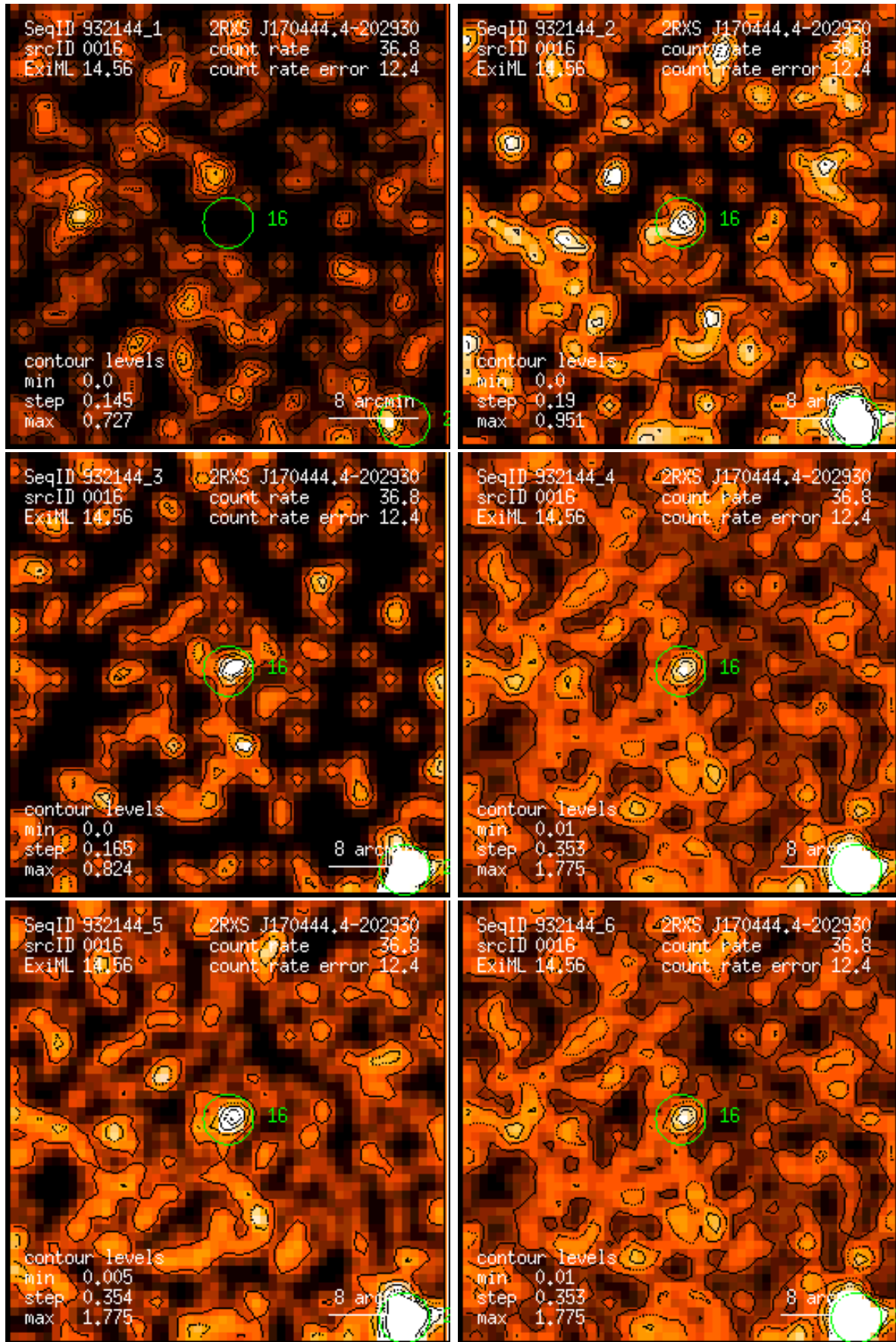
Figure 16: RASS 932144: detection 0016: band rate images, Gaussian filter: (1) PSPC channels 11 – 41, (2) 52 – 90, (3) 91 – 201, (4) 11 – 235, (5) 52 – 201, (6) 11 – 201. Broad band rates in counts/ks. Band rate contour levels in counts/ks/arcmin 2 .
