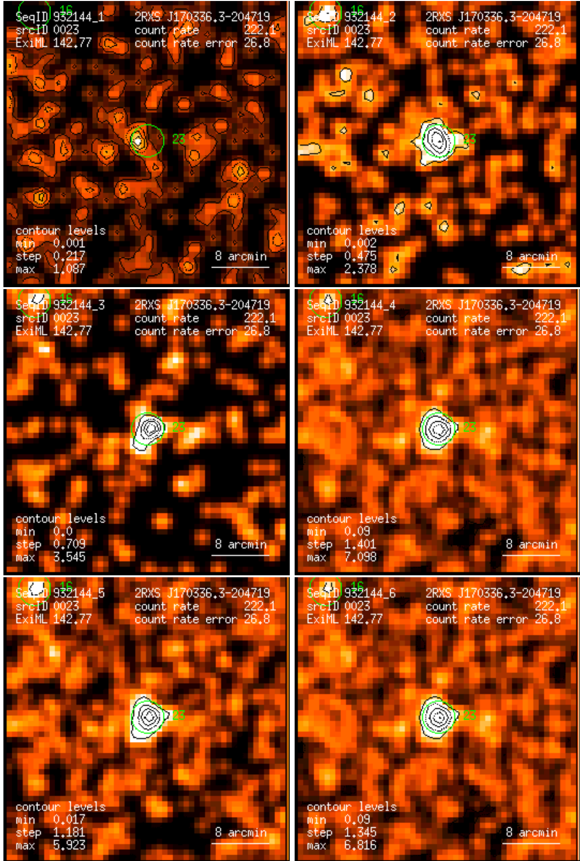
Figure 23: RASS 932144: detection 0023: band rate images, Gaussian filter: (1) PSPC channels 11 – 41, (2) 52 – 90, (3) 91 – 201, (4) 11 – 235, (5) 52 – 201, (6) 11 – 201. Broad band rates in counts/ks. Band rate contour levels in counts/ks/arcmin 2 .
