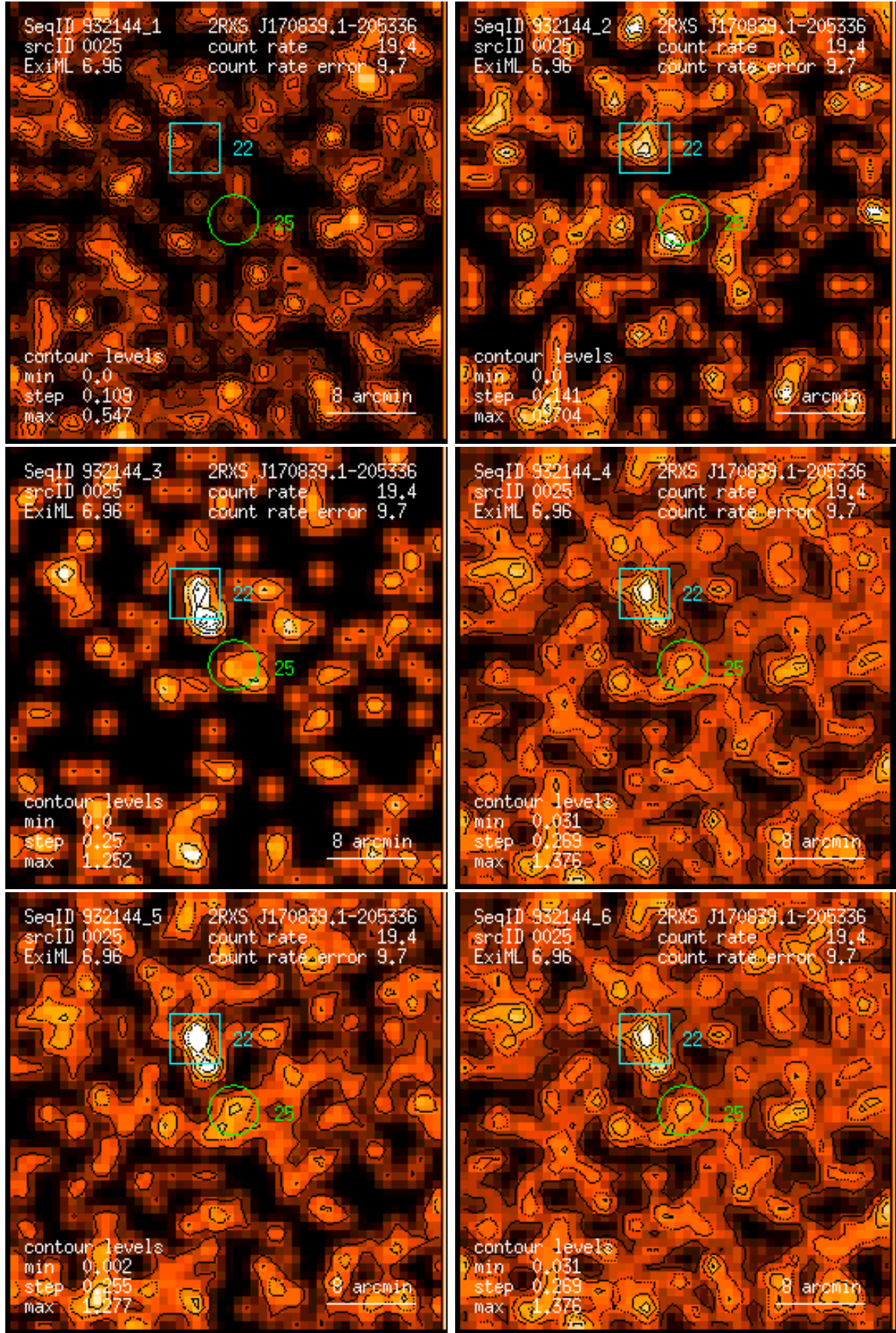
Figure 25: RASS 932144: detection 0025: band rate images, Gaussian filter: (1) PSPC channels 11 – 41, (2) 52 – 90, (3) 91 – 201, (4) 11 – 235, (5) 52 – 201, (6) 11 – 201. Broad band rates in counts/ks. Band rate contour levels in counts/ks/arcmin 2 .
