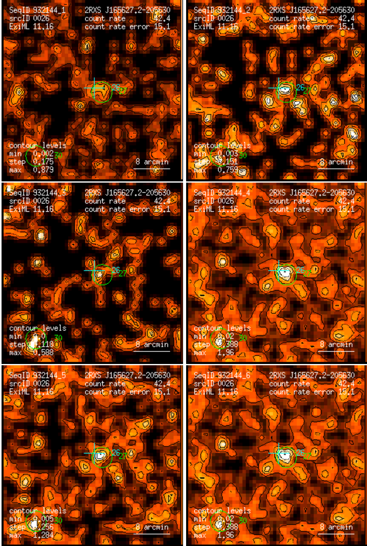
Figure 26: RASS 932144: detection 0026: band rate images, Gaussian filter: (1) PSPC channels 11 – 41, (2) 52 – 90, (3) 91 – 201, (4) 11 – 235, (5) 52 – 201, (6) 11 – 201. Broad band rates in counts/ks. Band rate contour levels in counts/ks/arcmin 2 .
