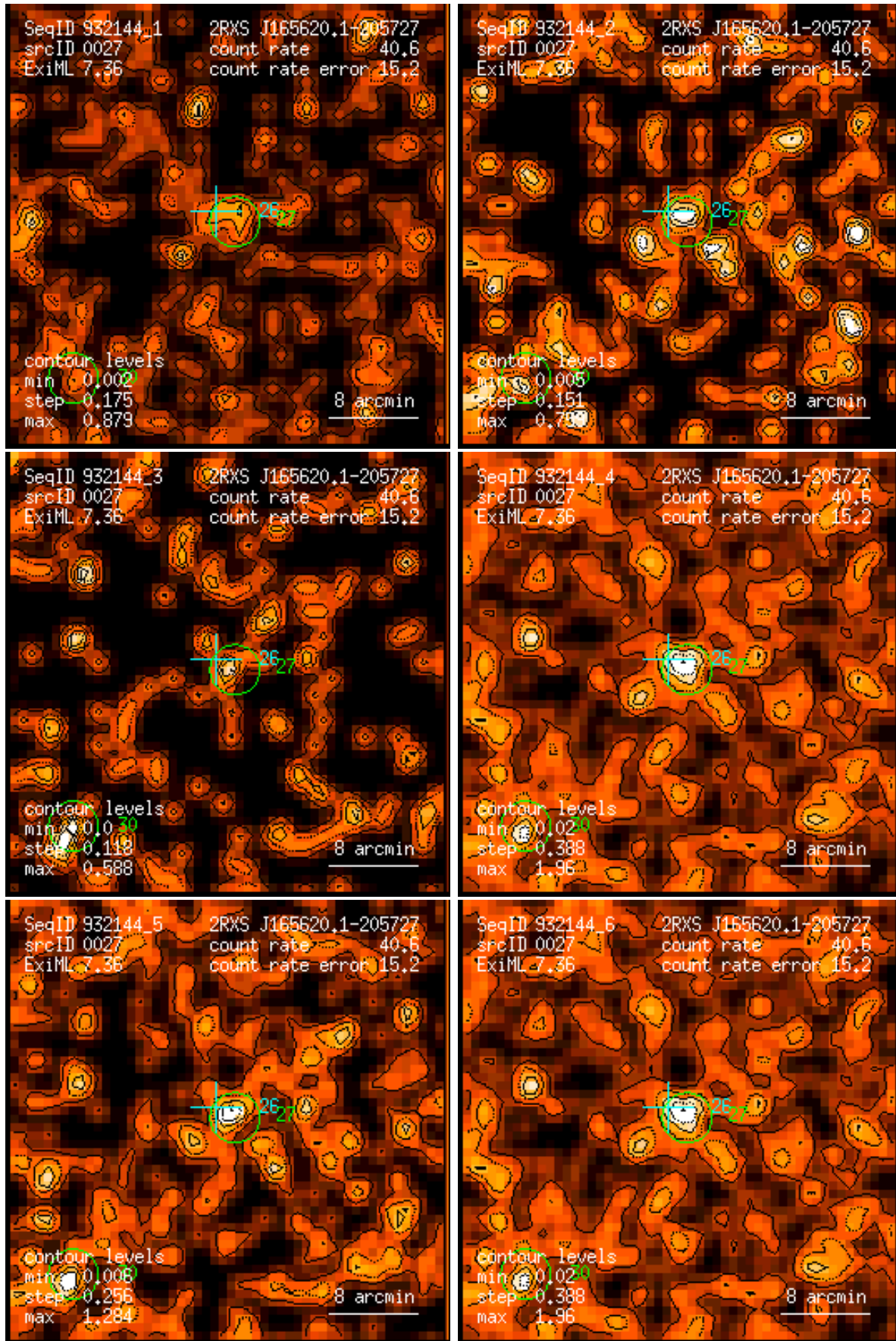
Figure 27: RASS 932144: detection 0027: band rate images, Gaussian filter: (1) PSPC channels 11 – 41, (2) 52 – 90, (3) 91 – 201, (4) 11 – 235, (5) 52 – 201, (6) 11 – 201. Broad band rates in counts/ks. Band rate contour levels in counts/ks/arcmin 2 .
