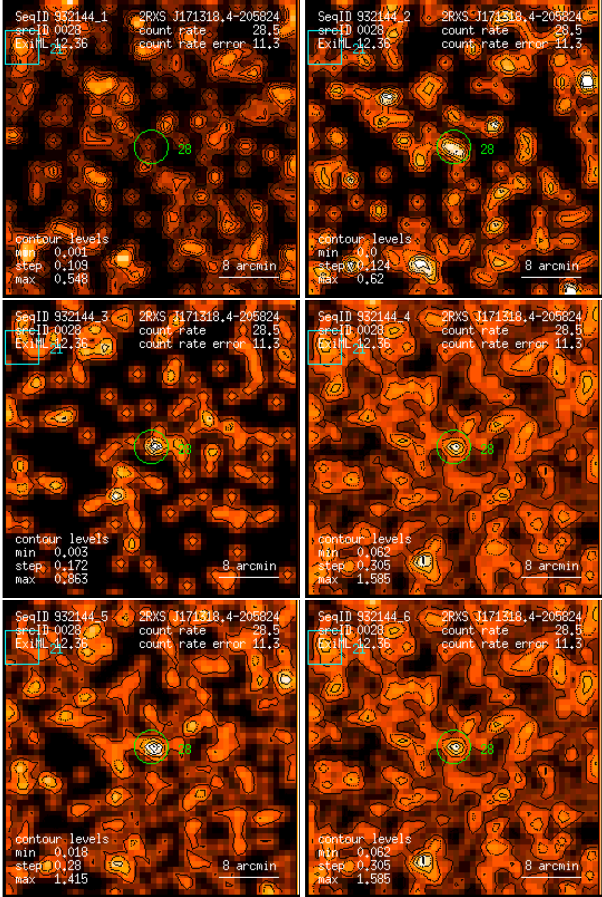
Figure 28: RASS 932144: detection 0028: band rate images, Gaussian filter: (1) PSPC channels 11 – 41, (2) 52 – 90, (3) 91 – 201, (4) 11 – 235, (5) 52 – 201, (6) 11 – 201. Broad band rates in counts/ks. Band rate contour levels in counts/ks/arcmin 2 .
