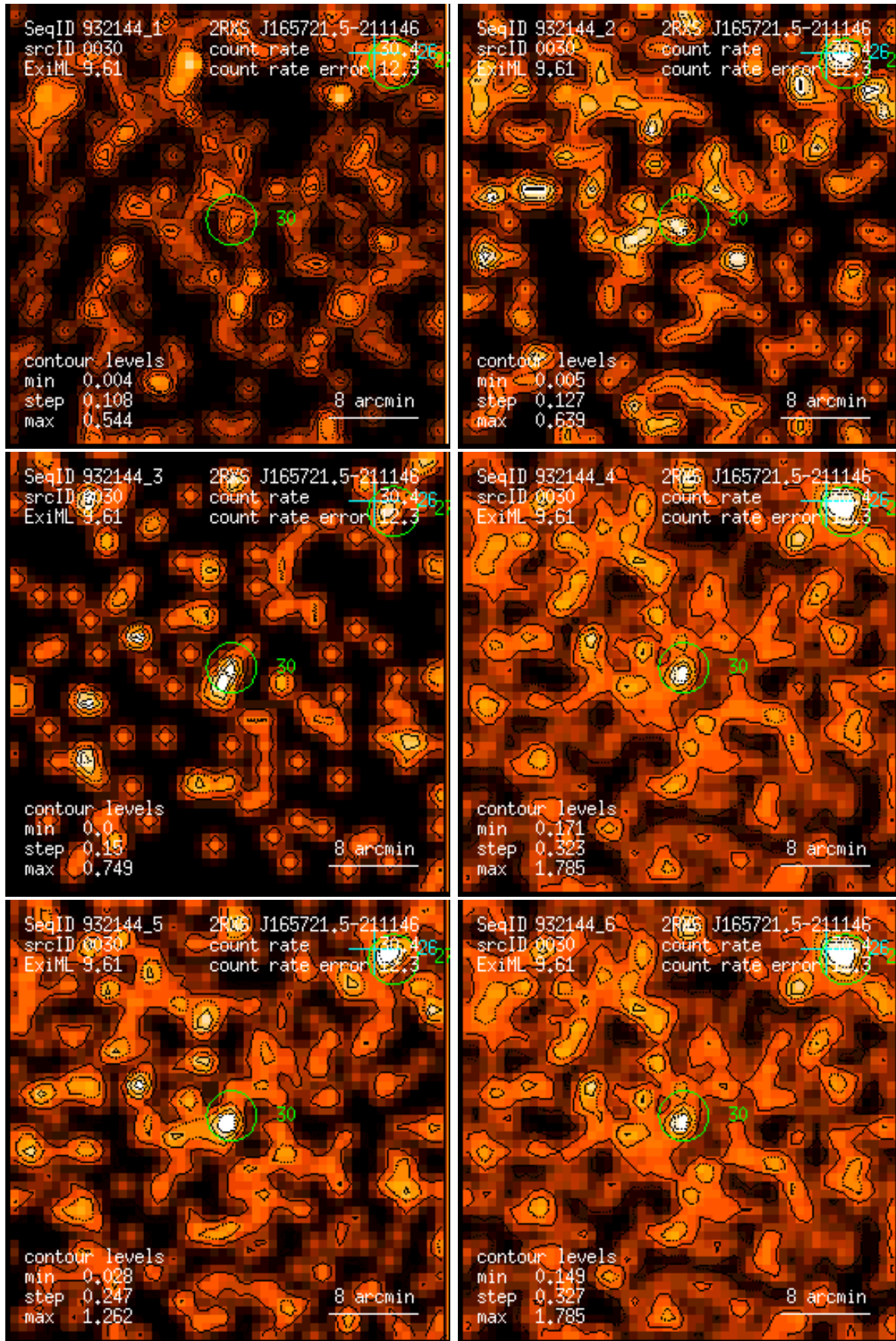
Figure 30: RASS 932144: detection 0030: band rate images, Gaussian filter: (1) PSPC channels 11 – 41, (2) 52 – 90, (3) 91 – 201, (4) 11 – 235, (5) 52 – 201, (6) 11 – 201. Broad band rates in counts/ks. Band rate contour levels in counts/ks/arcmin 2 .
