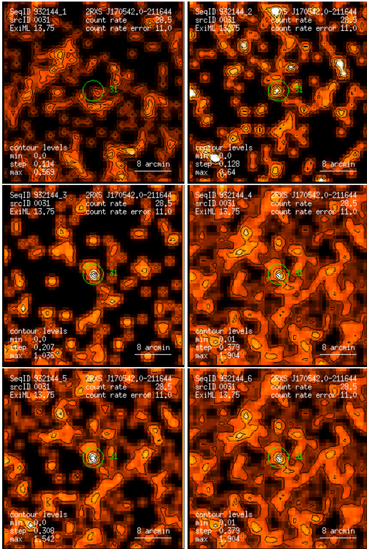
Figure 31: RASS 932144: detection 0031: band rate images, Gaussian filter: (1) PSPC channels 11 – 41, (2) 52 – 90, (3) 91 – 201, (4) 11 – 235, (5) 52 – 201, (6) 11 – 201. Broad band rates in counts/ks. Band rate contour levels in counts/ks/arcmin 2 .
