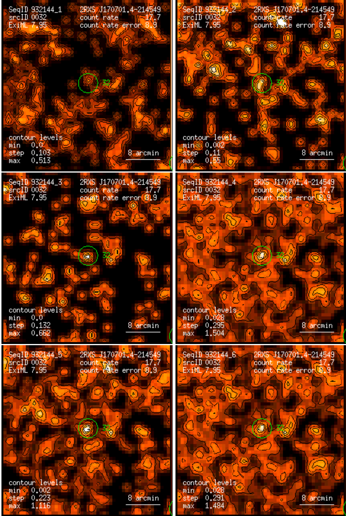
Figure 32: RASS 932144: detection 0032: band rate images, Gaussian filter: (1) PSPC channels 11 – 41, (2) 52 – 90, (3) 91 – 201, (4) 11 – 235, (5) 52 – 201, (6) 11 – 201. Broad band rates in counts/ks. Band rate contour levels in counts/ks/arcmin 2 .
