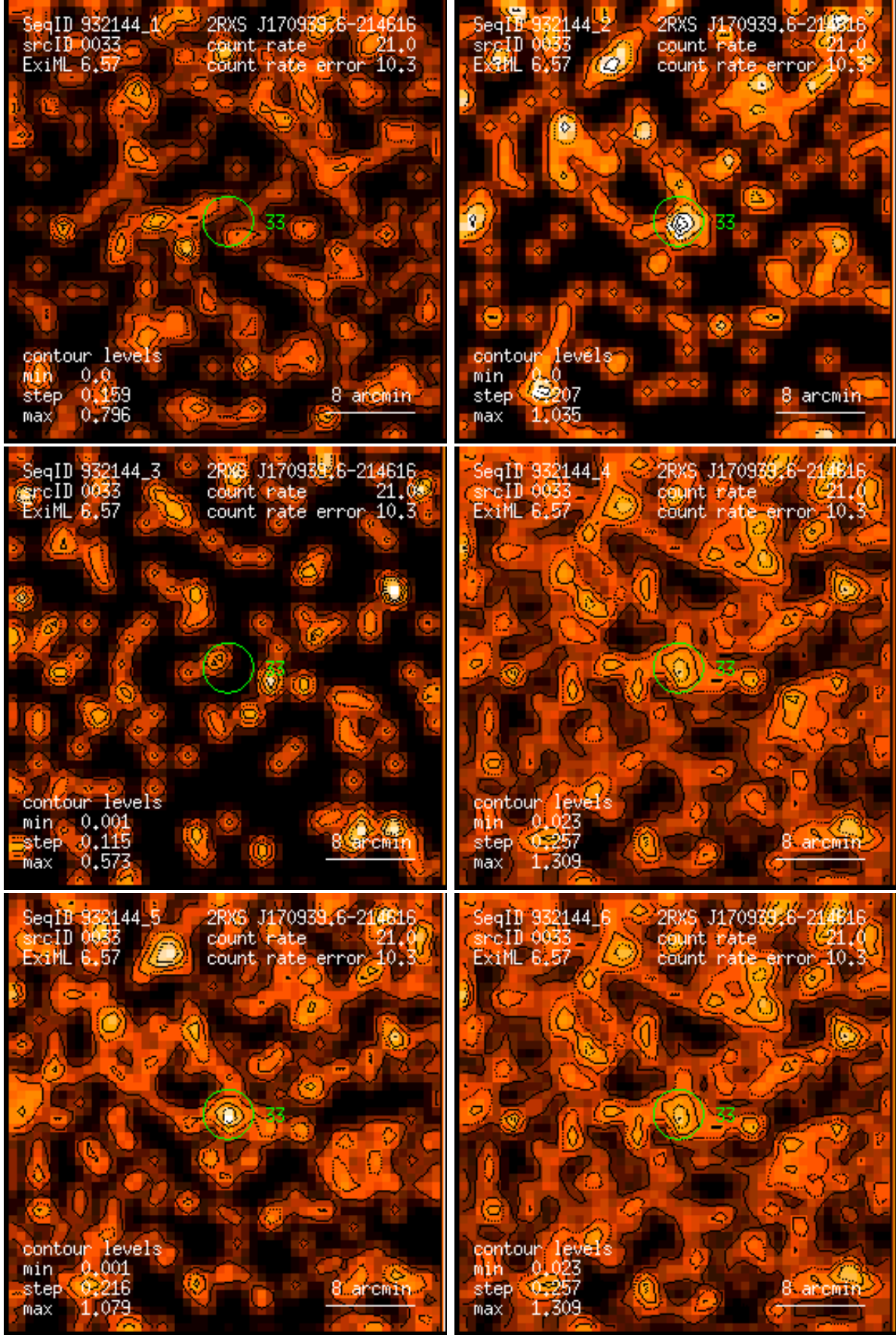
Figure 33: RASS 932144: detection 0033: band rate images, Gaussian filter: (1) PSPC channels 11 – 41, (2) 52 – 90, (3) 91 – 201, (4) 11 – 235, (5) 52 – 201, (6) 11 – 201. Broad band rates in counts/ks. Band rate contour levels in counts/ks/arcmin 2 .
