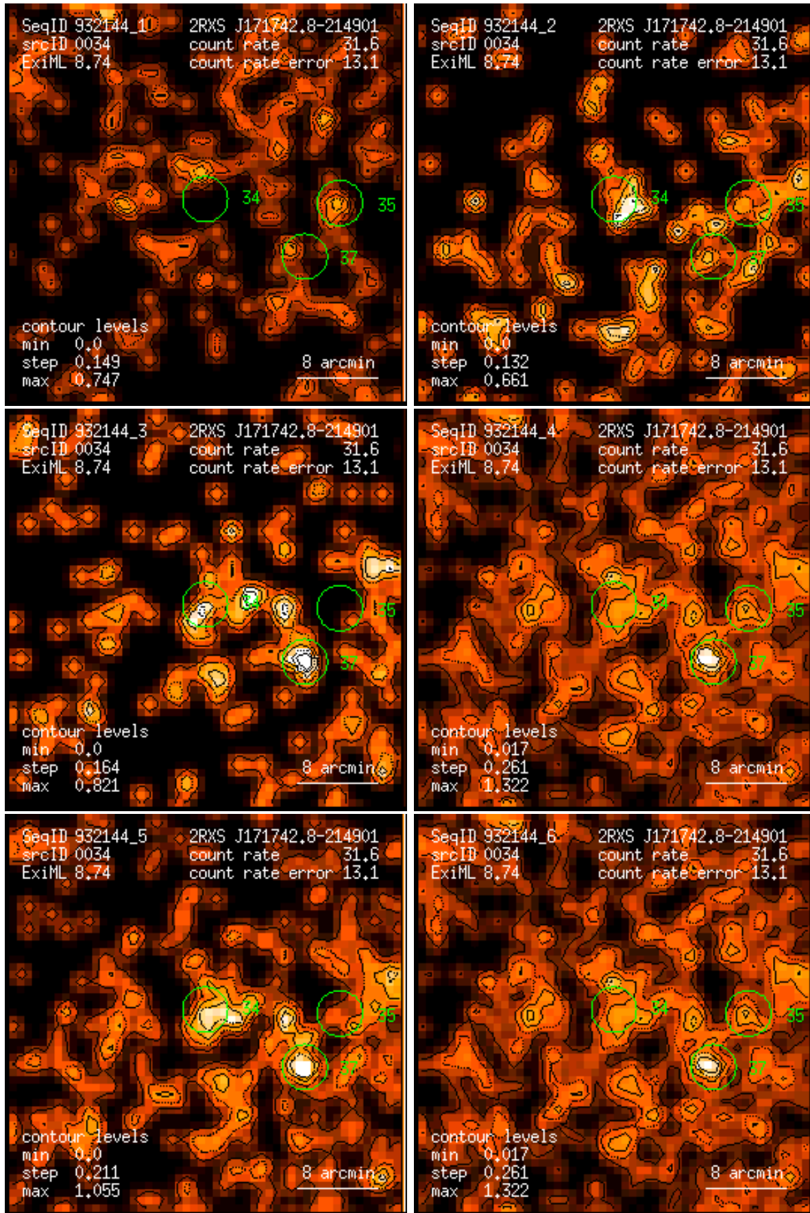
Figure 34: RASS 932144: detection 0034: band rate images, Gaussian filter: (1) PSPC channels 11 – 41, (2) 52 – 90, (3) 91 – 201, (4) 11 – 235, (5) 52 – 201, (6) 11 – 201. Broad band rates in counts/ks. Band rate contour levels in counts/ks/arcmin 2 .
