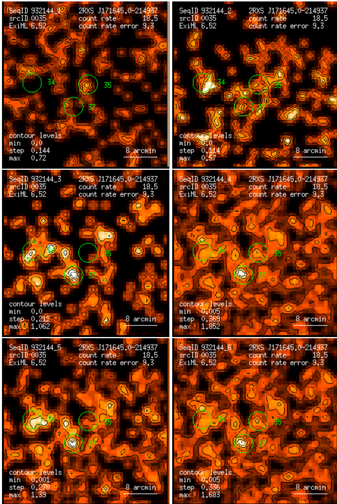
Figure 35: RASS 932144: detection 0035: band rate images, Gaussian filter: (1) PSPC channels 11 – 41, (2) 52 – 90, (3) 91 – 201, (4) 11 – 235, (5) 52 – 201, (6) 11 – 201. Broad band rates in counts/ks. Band rate contour levels in counts/ks/arcmin 2 .
