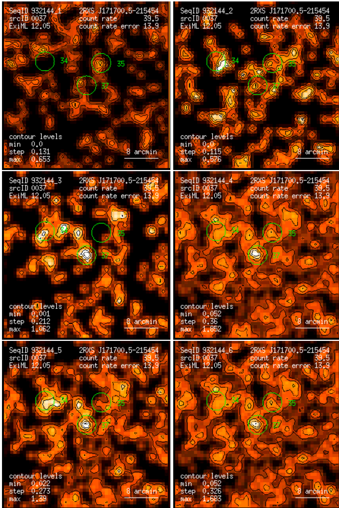
Figure 37: RASS 932144: detection 0037: band rate images, Gaussian filter: (1) PSPC channels 11 – 41, (2) 52 – 90, (3) 91 – 201, (4) 11 – 235, (5) 52 – 201, (6) 11 – 201. Broad band rates in counts/ks. Band rate contour levels in counts/ks/arcmin 2 .
