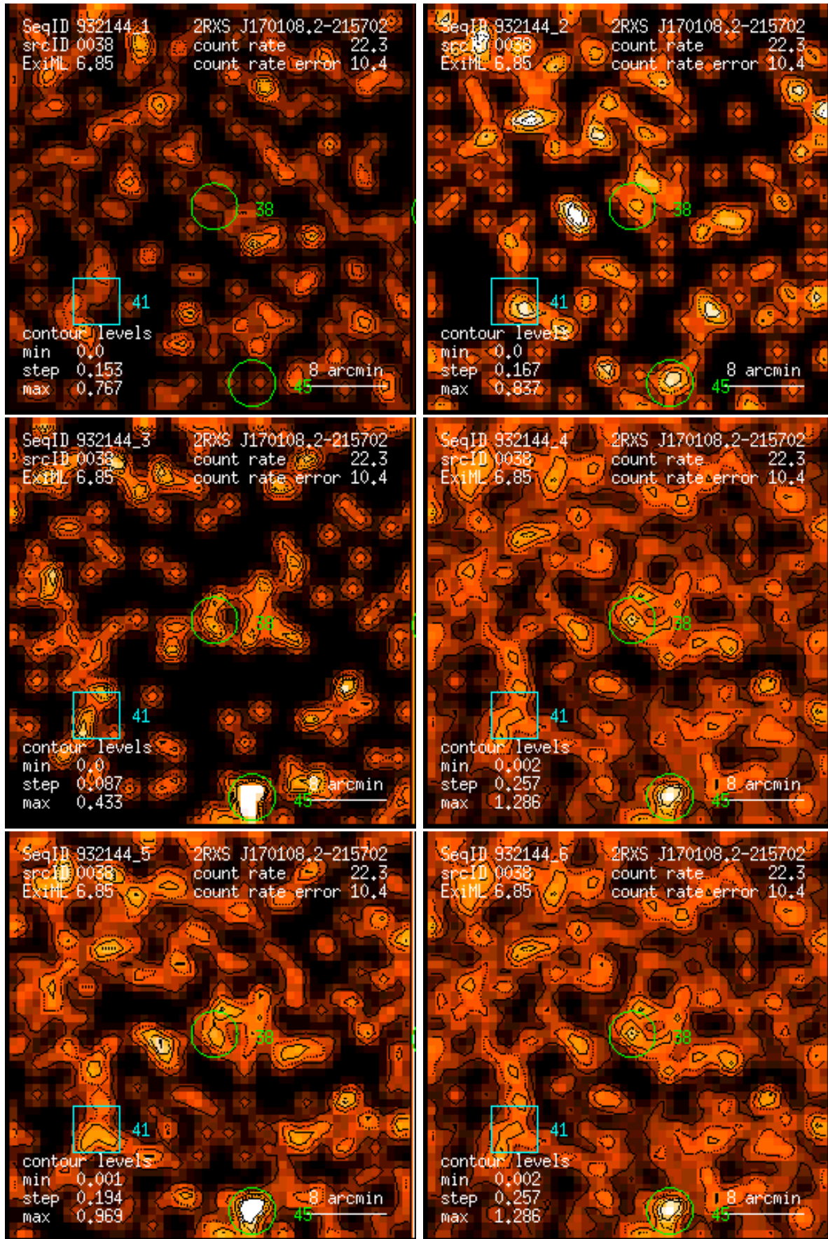
Figure 38: RASS 932144: detection 0038: band rate images, Gaussian filter: (1) PSPC channels 11 – 41, (2) 52 – 90, (3) 91 – 201, (4) 11 – 235, (5) 52 – 201, (6) 11 – 201. Broad band rates in counts/ks. Band rate contour levels in counts/ks/arcmin 2 .
