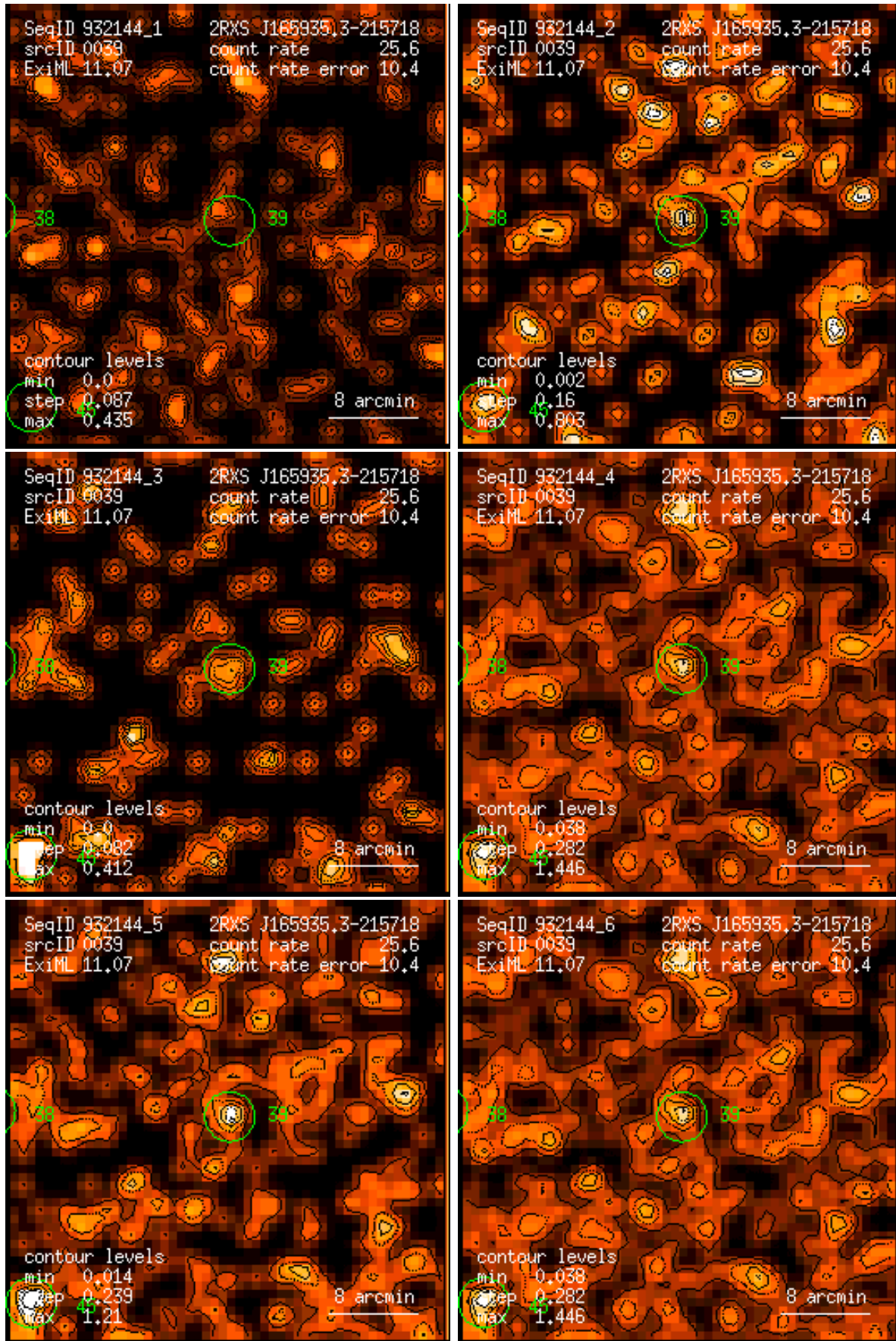
Figure 39: RASS 932144: detection 0039: band rate images, Gaussian filter: (1) PSPC channels 11 – 41, (2) 52 – 90, (3) 91 – 201, (4) 11 – 235, (5) 52 – 201, (6) 11 – 201. Broad band rates in counts/ks. Band rate contour levels in counts/ks/arcmin 2 .
