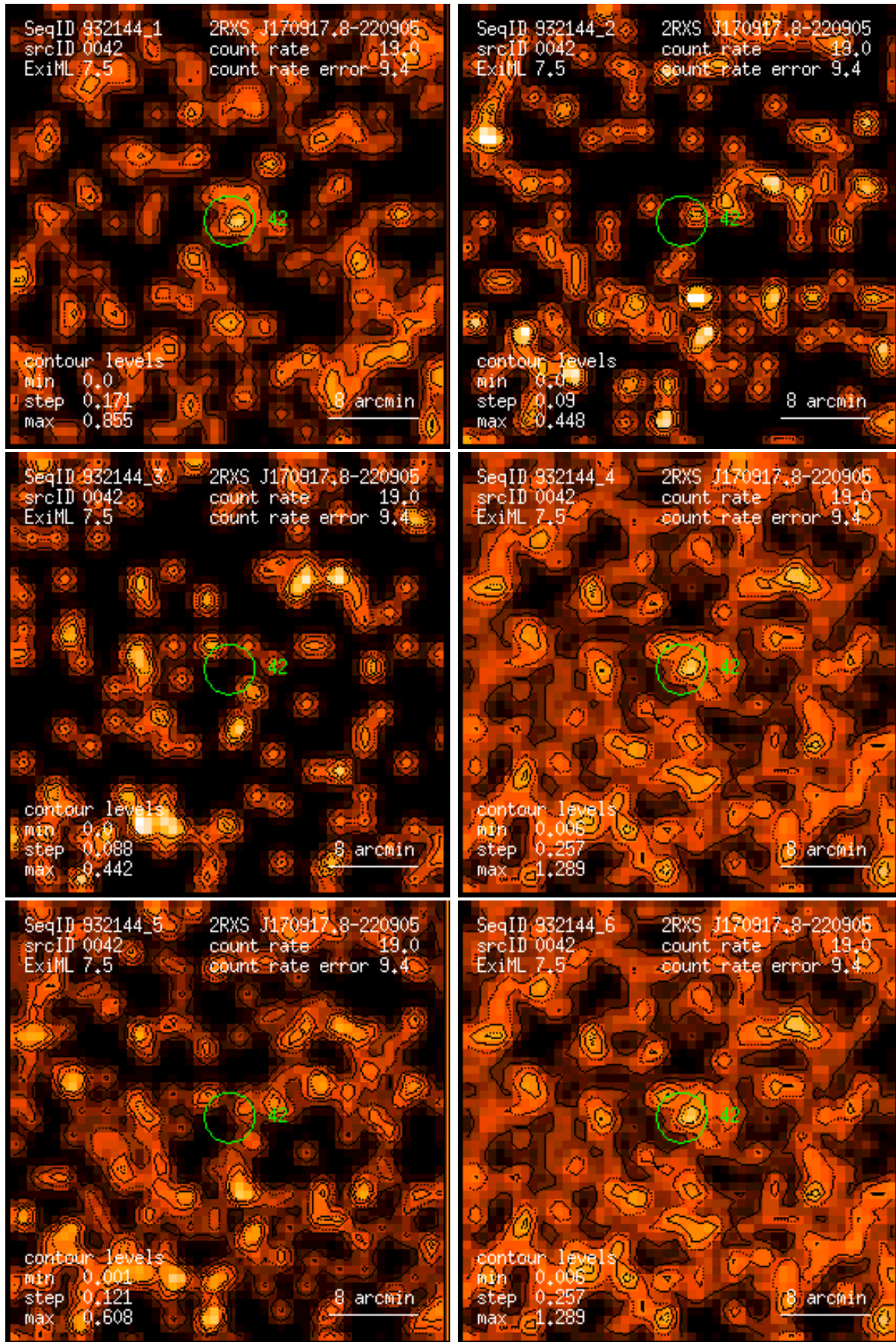
Figure 42: RASS 932144: detection 0042: band rate images, Gaussian filter: (1) PSPC channels 11 – 41, (2) 52 – 90, (3) 91 – 201, (4) 11 – 235, (5) 52 – 201, (6) 11 – 201. Broad band rates in counts/ks. Band rate contour levels in counts/ks/arcmin 2 .
