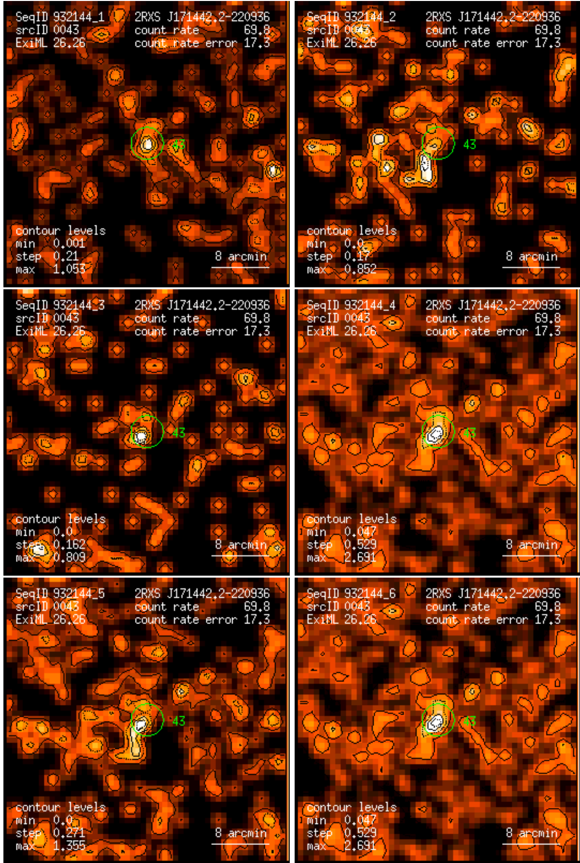
Figure 43: RASS 932144: detection 0043: band rate images, Gaussian filter: (1) PSPC channels 11 – 41, (2) 52 – 90, (3) 91 – 201, (4) 11 – 235, (5) 52 – 201, (6) 11 – 201. Broad band rates in counts/ks. Band rate contour levels in counts/ks/arcmin 2 .
