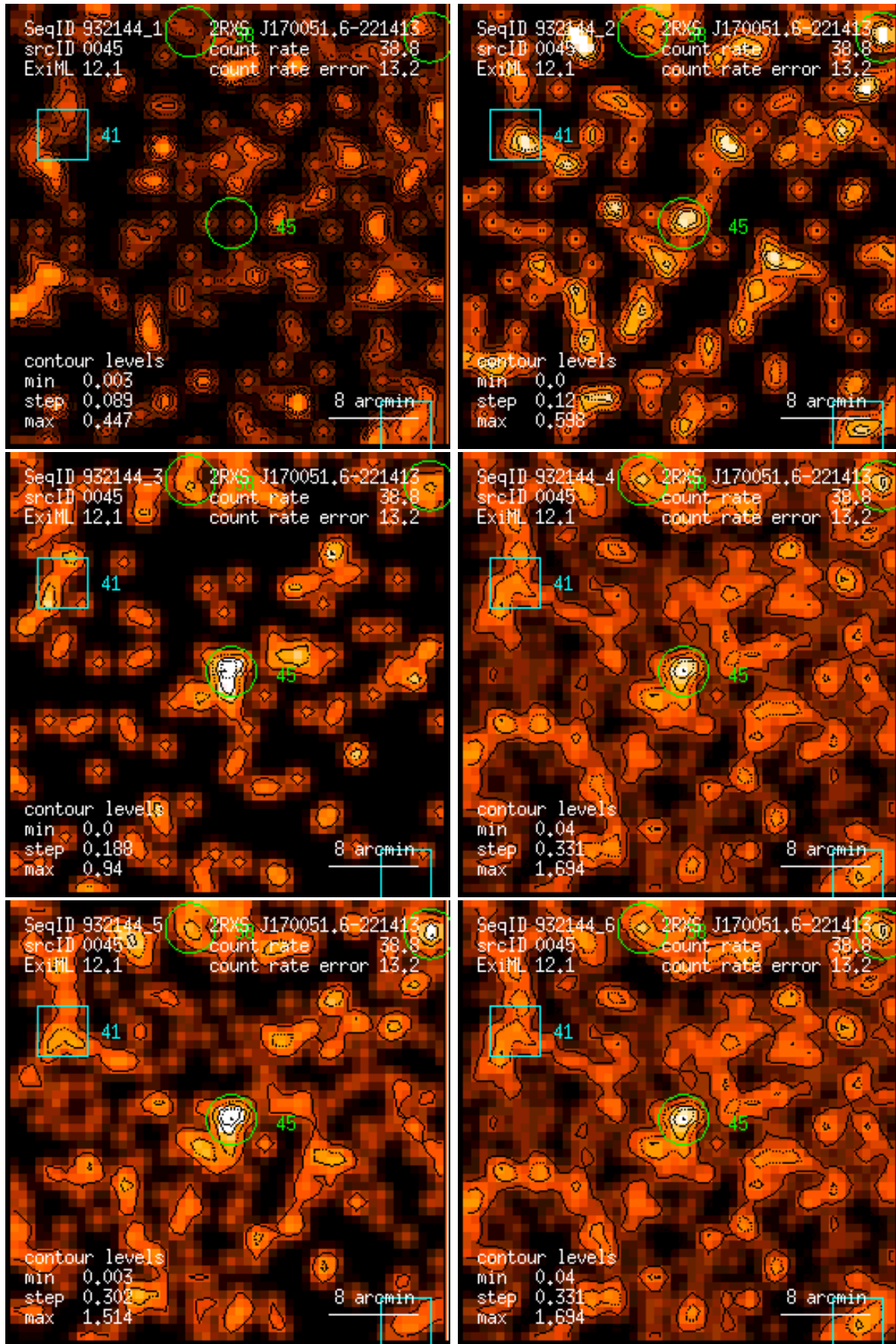
Figure 45: RASS 932144: detection 0045: band rate images, Gaussian filter: (1) PSPC channels 11 – 41, (2) 52 – 90, (3) 91 – 201, (4) 11 – 235, (5) 52 – 201, (6) 11 – 201. Broad band rates in counts/ks. Band rate contour levels in counts/ks/arcmin 2 .
