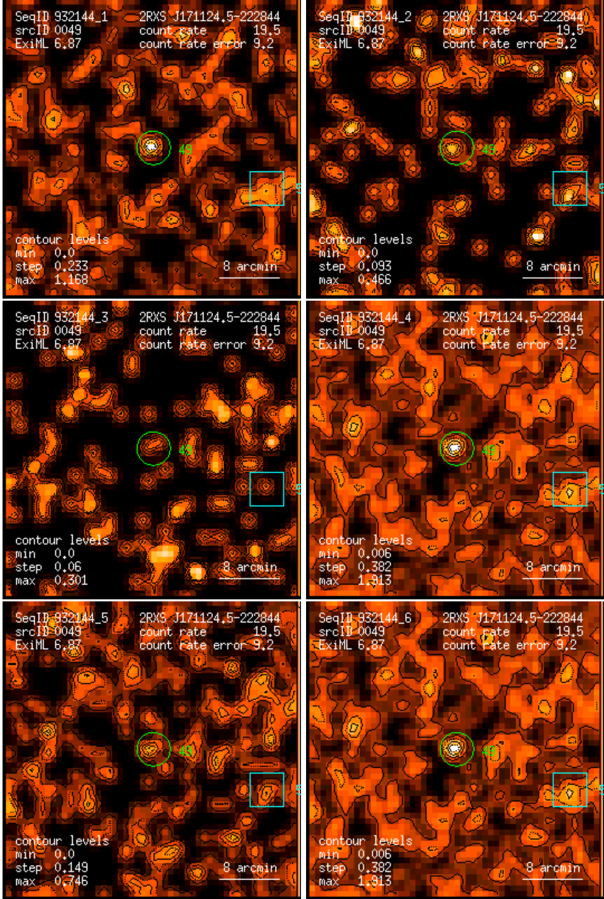
Figure 49: RASS 932144: detection 0049: band rate images, Gaussian filter: (1) PSPC channels 11 – 41, (2) 52 – 90, (3) 91 – 201, (4) 11 – 235, (5) 52 – 201, (6) 11 – 201. Broad band rates in counts/ks. Band rate contour levels in counts/ks/arcmin 2 .
