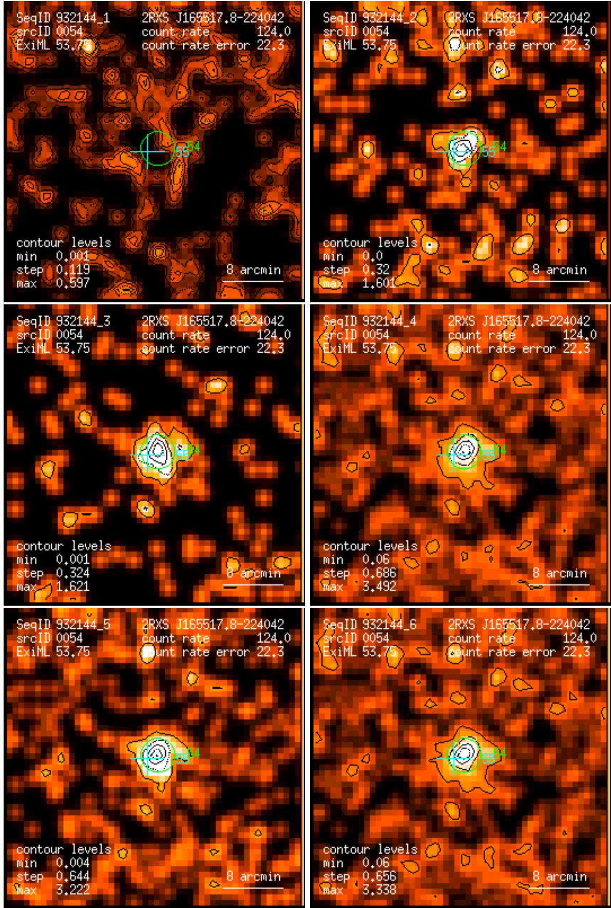
Figure 54: RASS 932144: detection 0054: band rate images, Gaussian filter: (1) PSPC channels 11 – 41, (2) 52 – 90, (3) 91 – 201, (4) 11 – 235, (5) 52 – 201, (6) 11 – 201. Broad band rates in counts/ks. Band rate contour levels in counts/ks/arcmin 2 .
