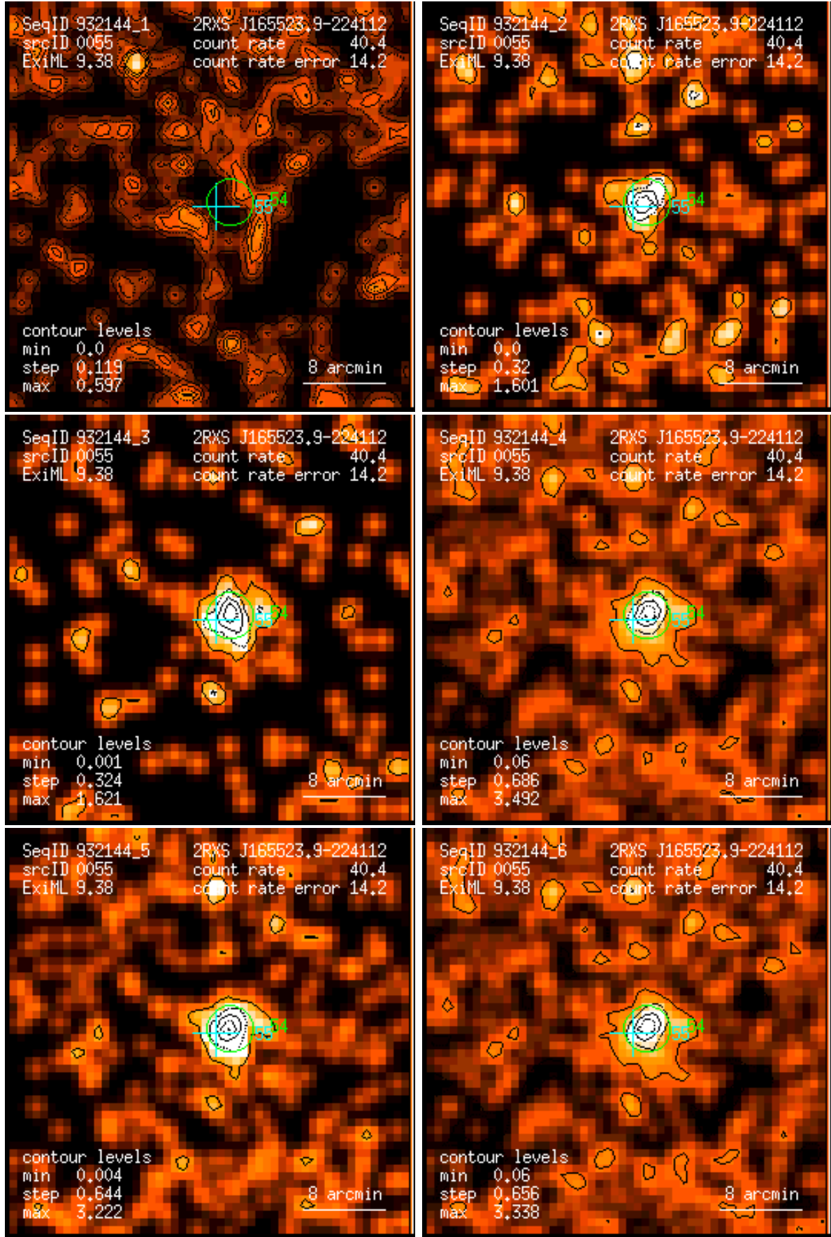
Figure 55: RASS 932144: detection 0055: band rate images, Gaussian filter: (1) PSPC channels 11 – 41, (2) 52 – 90, (3) 91 – 201, (4) 11 – 235, (5) 52 – 201, (6) 11 – 201. Broad band rates in counts/ks. Band rate contour levels in counts/ks/arcmin 2 .
