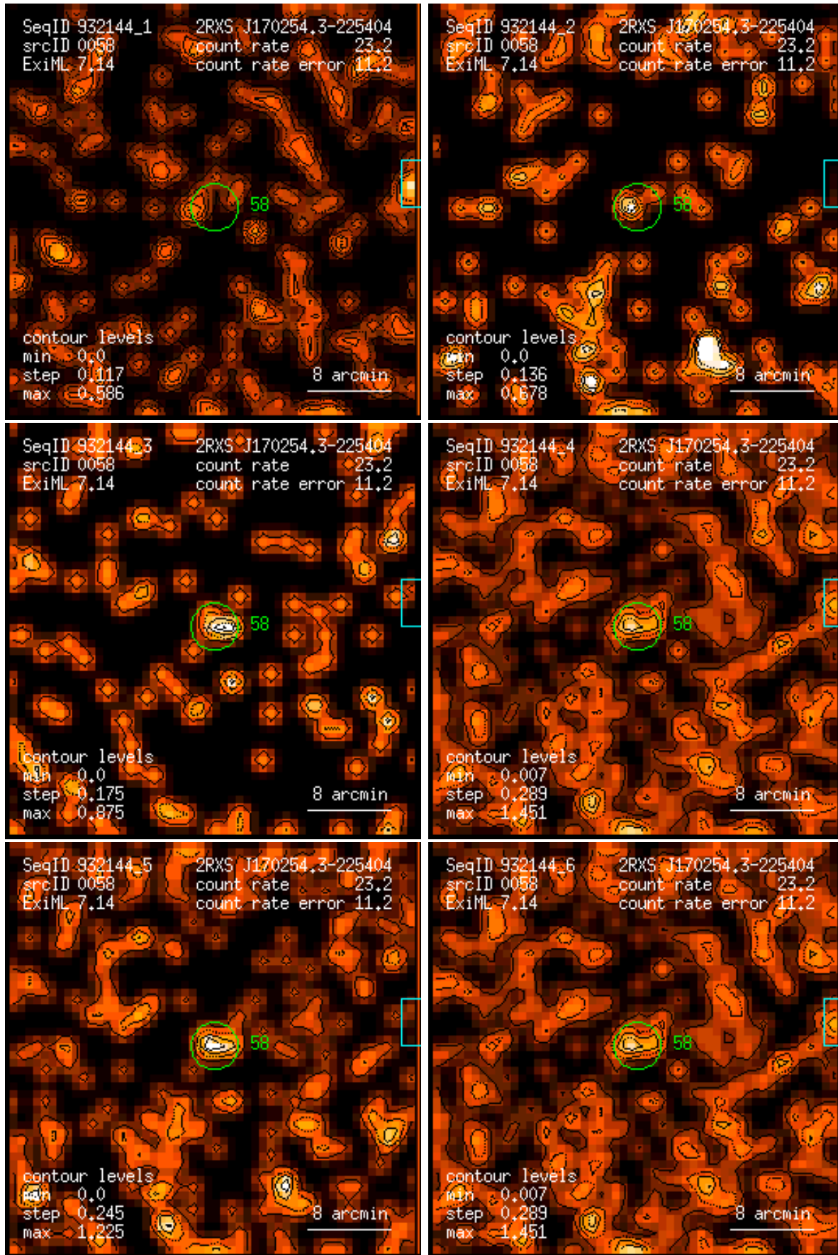
Figure 58: RASS 932144: detection 0058: band rate images, Gaussian filter: (1) PSPC channels 11 – 41, (2) 52 – 90, (3) 91 – 201, (4) 11 – 235, (5) 52 – 201, (6) 11 – 201. Broad band rates in counts/ks. Band rate contour levels in counts/ks/arcmin 2 .
