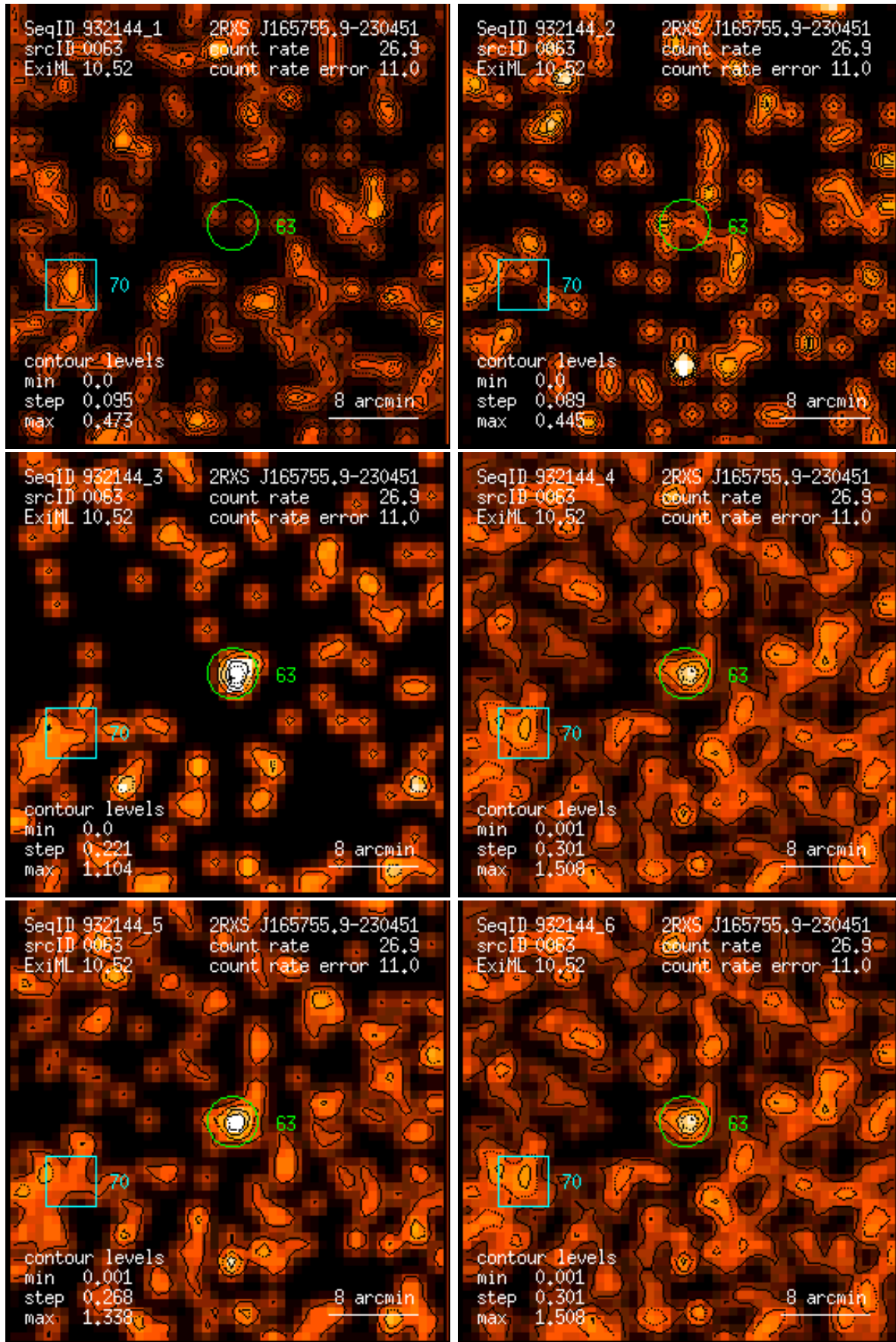
Figure 63: RASS 932144: detection 0063: band rate images, Gaussian filter: (1) PSPC channels 11 – 41, (2) 52 – 90, (3) 91 – 201, (4) 11 – 235, (5) 52 – 201, (6) 11 – 201. Broad band rates in counts/ks. Band rate contour levels in counts/ks/arcmin 2 .
