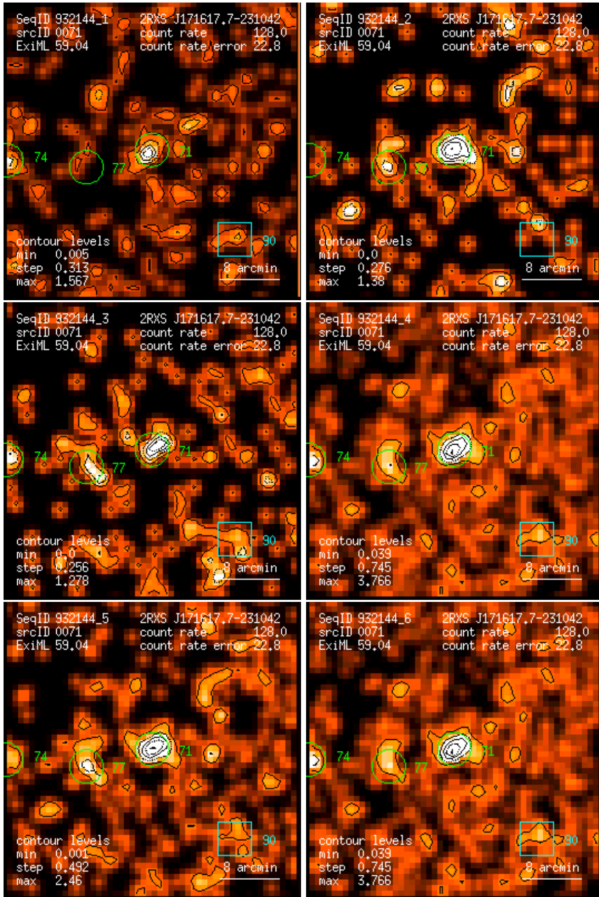
Figure 71: RASS 932144: detection 0071: band rate images, Gaussian filter: (1) PSPC channels 11 – 41, (2) 52 – 90, (3) 91 – 201, (4) 11 – 235, (5) 52 – 201, (6) 11 – 201. Broad band rates in counts/ks. Band rate contour levels in counts/ks/arcmin 2 .
