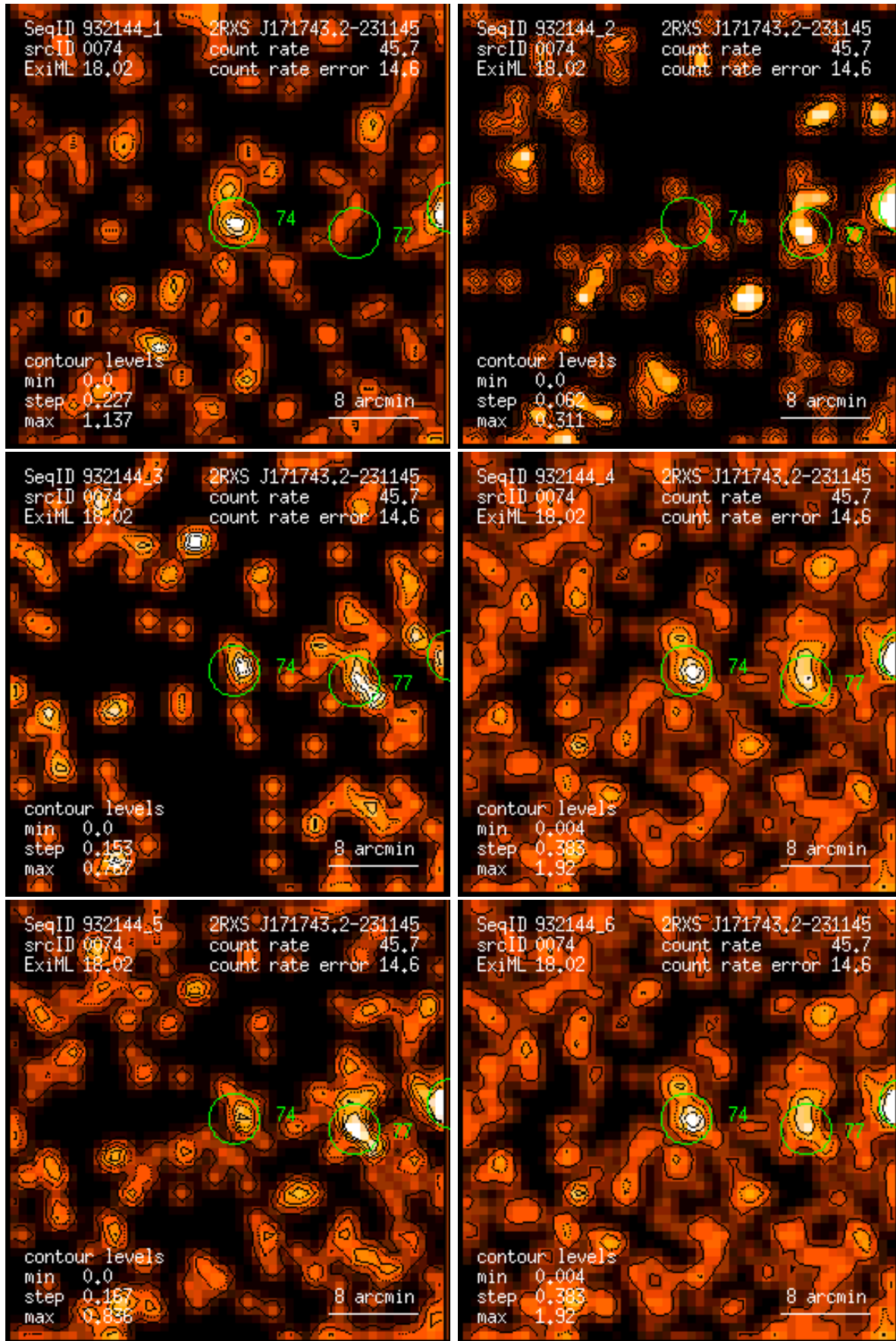
Figure 74: RASS 932144: detection 0074: band rate images, Gaussian filter: (1) PSPC channels 11 – 41, (2) 52 – 90, (3) 91 – 201, (4) 11 – 235, (5) 52 – 201, (6) 11 – 201. Broad band rates in counts/ks. Band rate contour levels in counts/ks/arcmin 2 .
