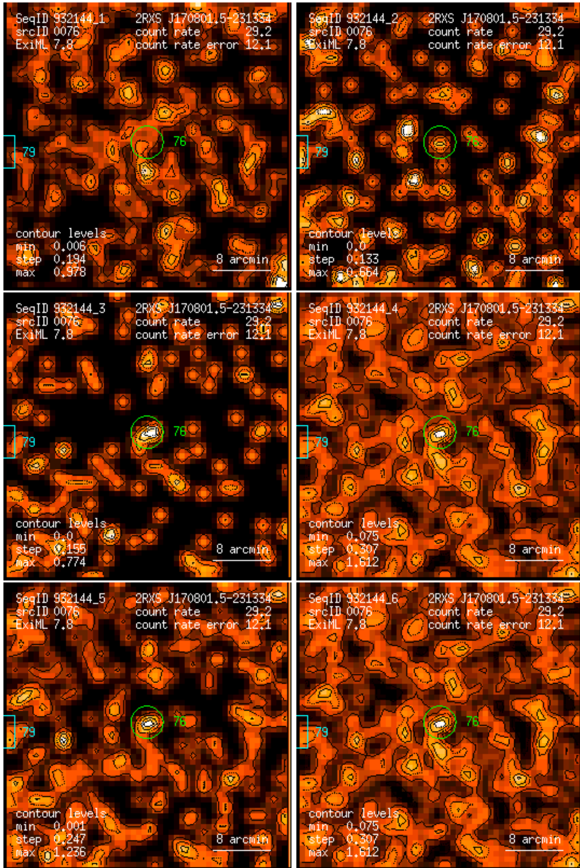
Figure 76: RASS 932144: detection 0076: band rate images, Gaussian filter: (1) PSPC channels 11 – 41, (2) 52 – 90, (3) 91 – 201, (4) 11 – 235, (5) 52 – 201, (6) 11 – 201. Broad band rates in counts/ks. Band rate contour levels in counts/ks/arcmin 2 .
