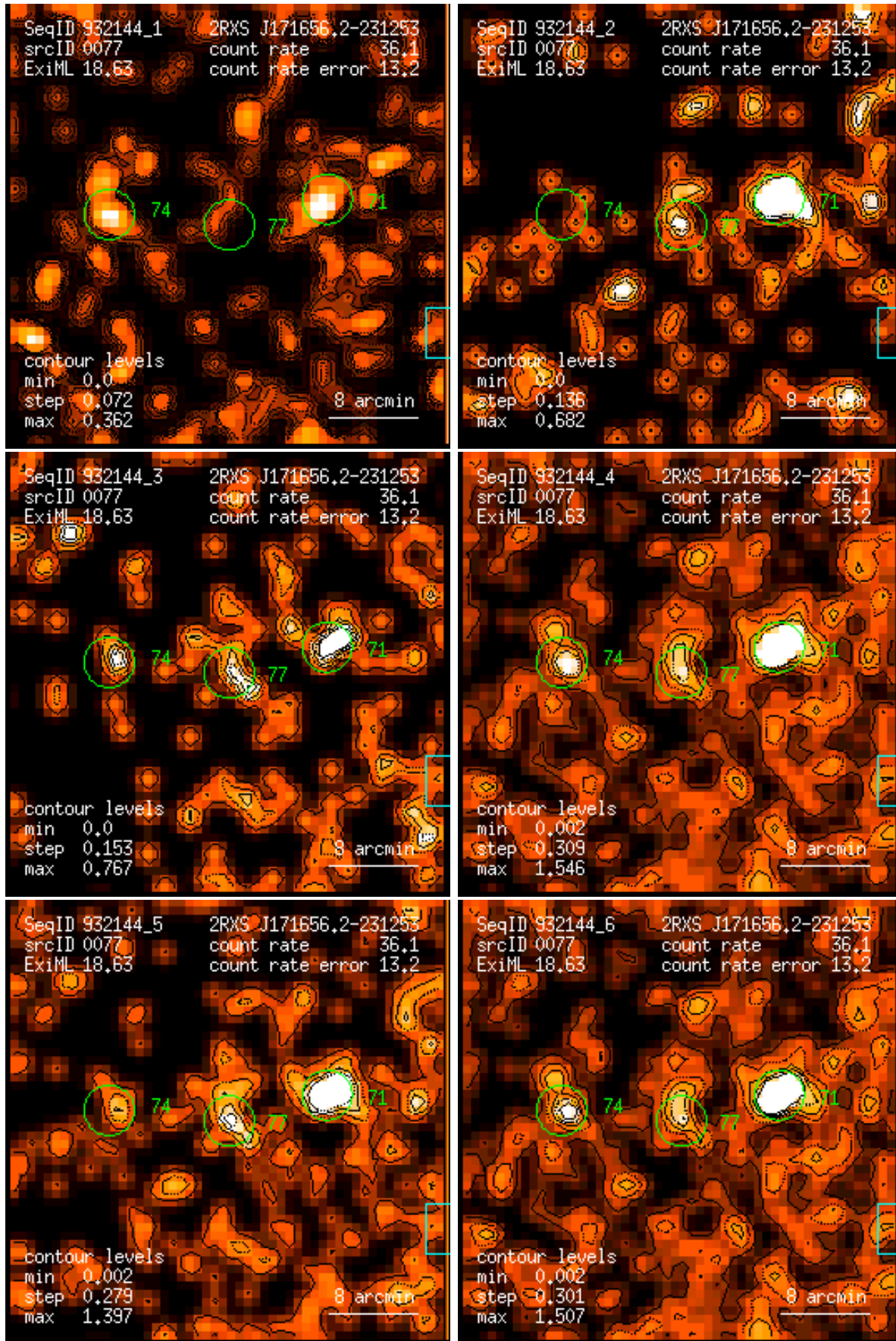
Figure 77: RASS 932144: detection 0077: band rate images, Gaussian filter: (1) PSPC channels 11 – 41, (2) 52 – 90, (3) 91 – 201, (4) 11 – 235, (5) 52 – 201, (6) 11 – 201. Broad band rates in counts/ks. Band rate contour levels in counts/ks/arcmin 2 .
