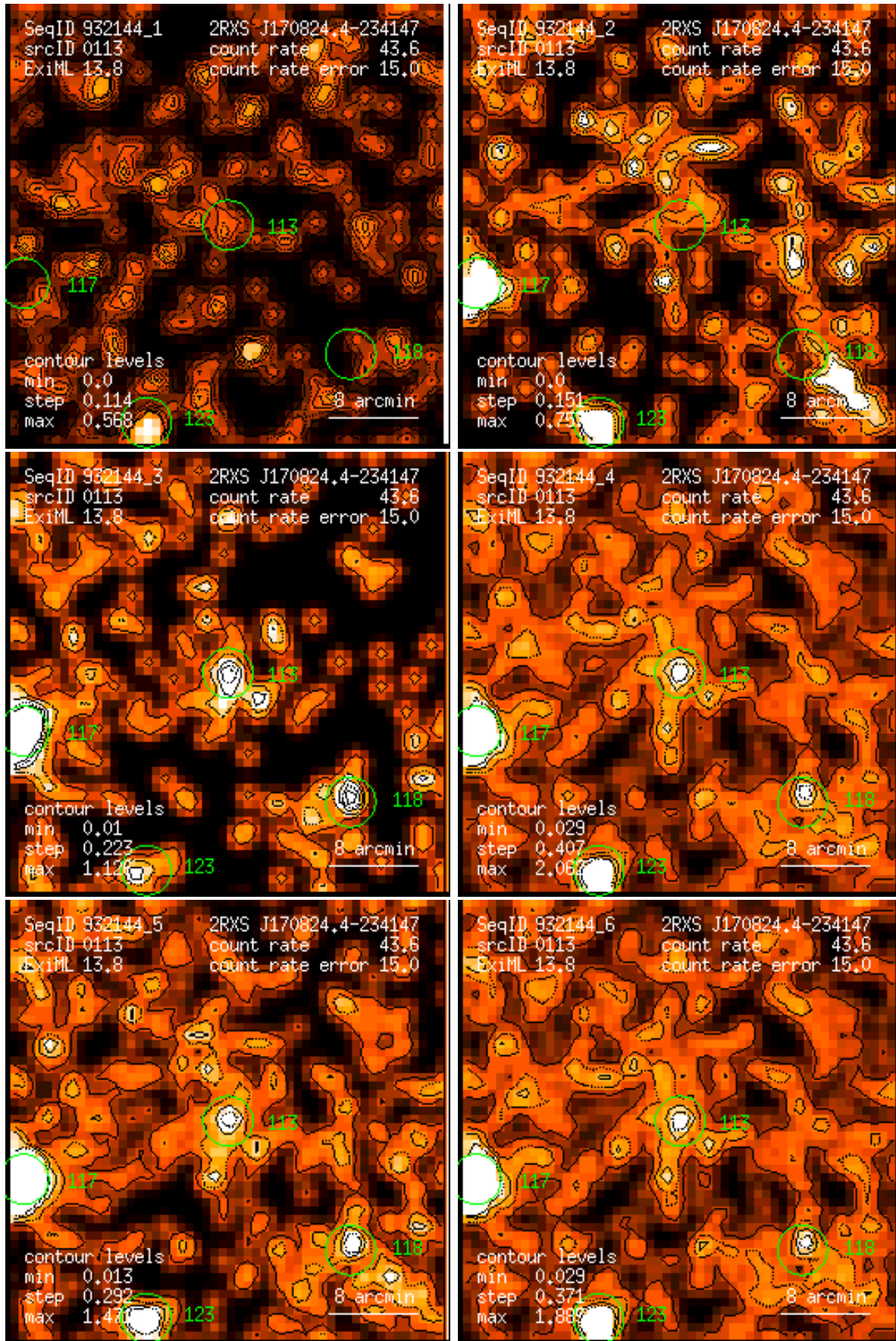
Figure 113: RASS 932144: detection 0113: band rate images, Gaussian filter: (1) PSPC channels 11 – 41, (2) 52 – 90, (3) 91 – 201, (4) 11 – 235, (5) 52 – 201, (6) 11 – 201. Broad band rates in counts/ks. Band rate contour levels in counts/ks/arcmin 2 .
