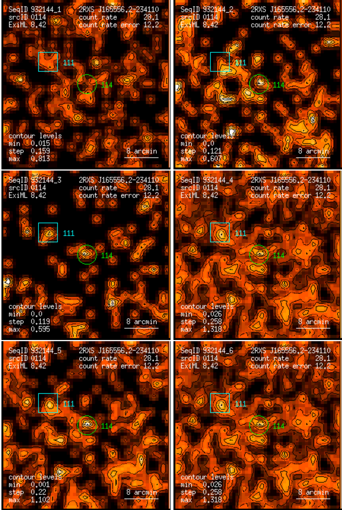
Figure 114: RASS 932144: detection 0114: band rate images, Gaussian filter: (1) PSPC channels 11 – 41, (2) 52 – 90, (3) 91 – 201, (4) 11 – 235, (5) 52 – 201, (6) 11 – 201. Broad band rates in counts/ks. Band rate contour levels in counts/ks/arcmin 2 .
