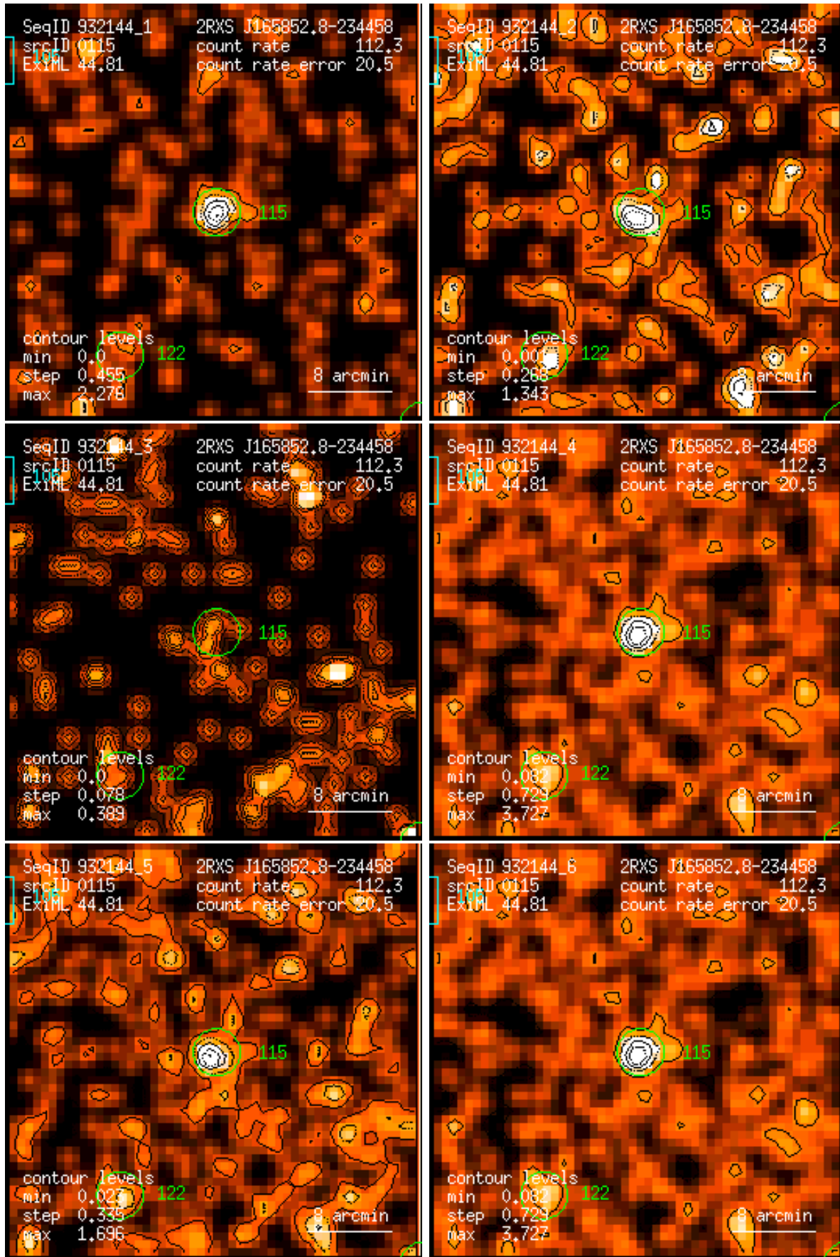
Figure 115: RASS 932144: detection 0115: band rate images, Gaussian filter: (1) PSPC channels 11 – 41, (2) 52 – 90, (3) 91 – 201, (4) 11 – 235, (5) 52 – 201, (6) 11 – 201. Broad band rates in counts/ks. Band rate contour levels in counts/ks/arcmin 2 .
