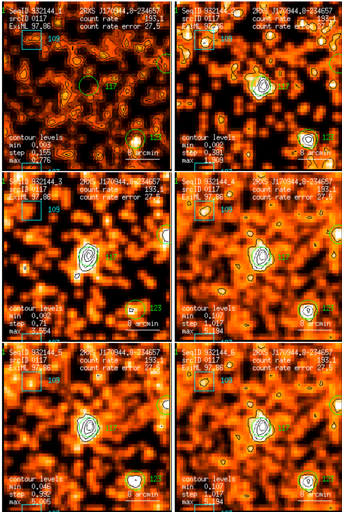
Figure 117: RASS 932144: detection 0117: band rate images, Gaussian filter: (1) PSPC channels 11 – 41, (2) 52 – 90, (3) 91 – 201, (4) 11 – 235, (5) 52 – 201, (6) 11 – 201. Broad band rates in counts/ks. Band rate contour levels in counts/ks/arcmin 2 .
