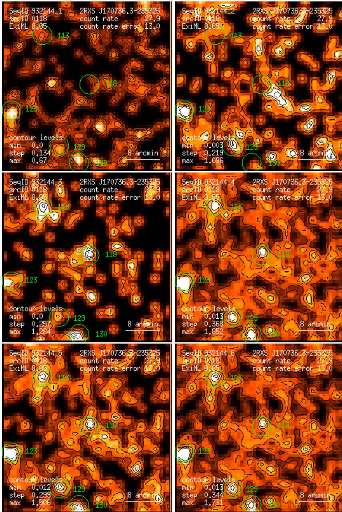
Figure 118: RASS 932144: detection 0118: band rate images, Gaussian filter: (1) PSPC channels 11 – 41, (2) 52 – 90, (3) 91 – 201, (4) 11 – 235, (5) 52 – 201, (6) 11 – 201. Broad band rates in counts/ks. Band rate contour levels in counts/ks/arcmin 2 .
