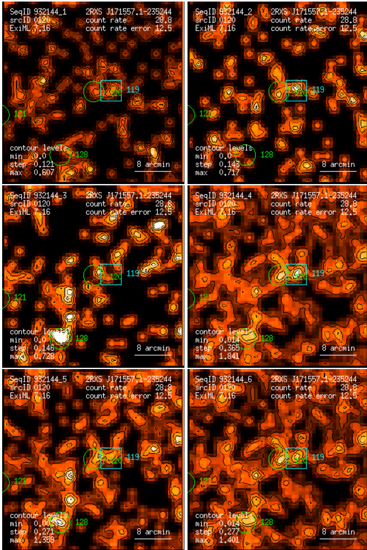
Figure 120: RASS 932144: detection 0120: band rate images, Gaussian filter: (1) PSPC channels 11 – 41, (2) 52 – 90, (3) 91 – 201, (4) 11 – 235, (5) 52 – 201, (6) 11 – 201. Broad band rates in counts/ks. Band rate contour levels in counts/ks/arcmin 2 .
