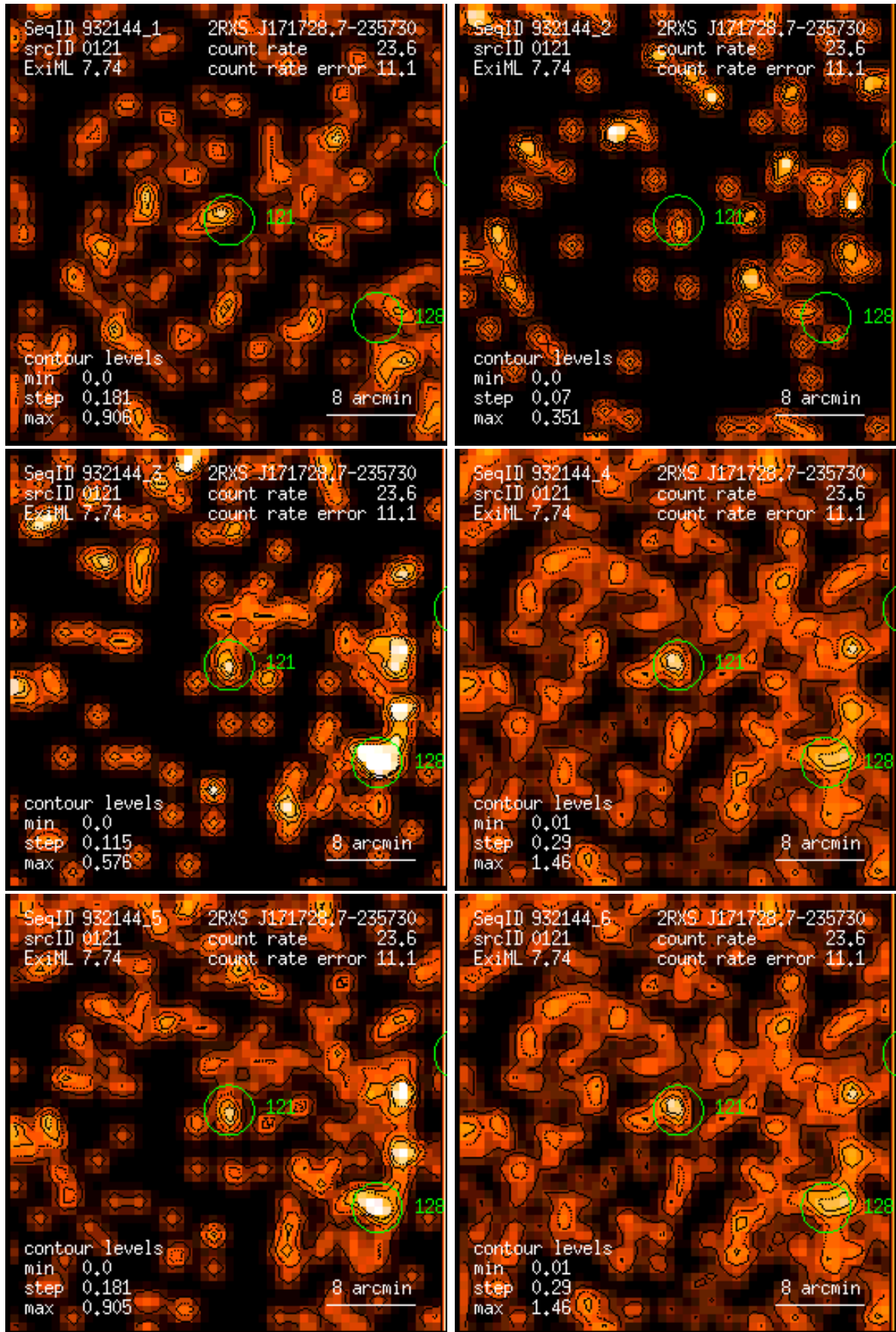
Figure 121: RASS 932144: detection 0121: band rate images, Gaussian filter: (1) PSPC channels 11 – 41, (2) 52 – 90, (3) 91 – 201, (4) 11 – 235, (5) 52 – 201, (6) 11 – 201. Broad band rates in counts/ks. Band rate contour levels in counts/ks/arcmin 2 .
