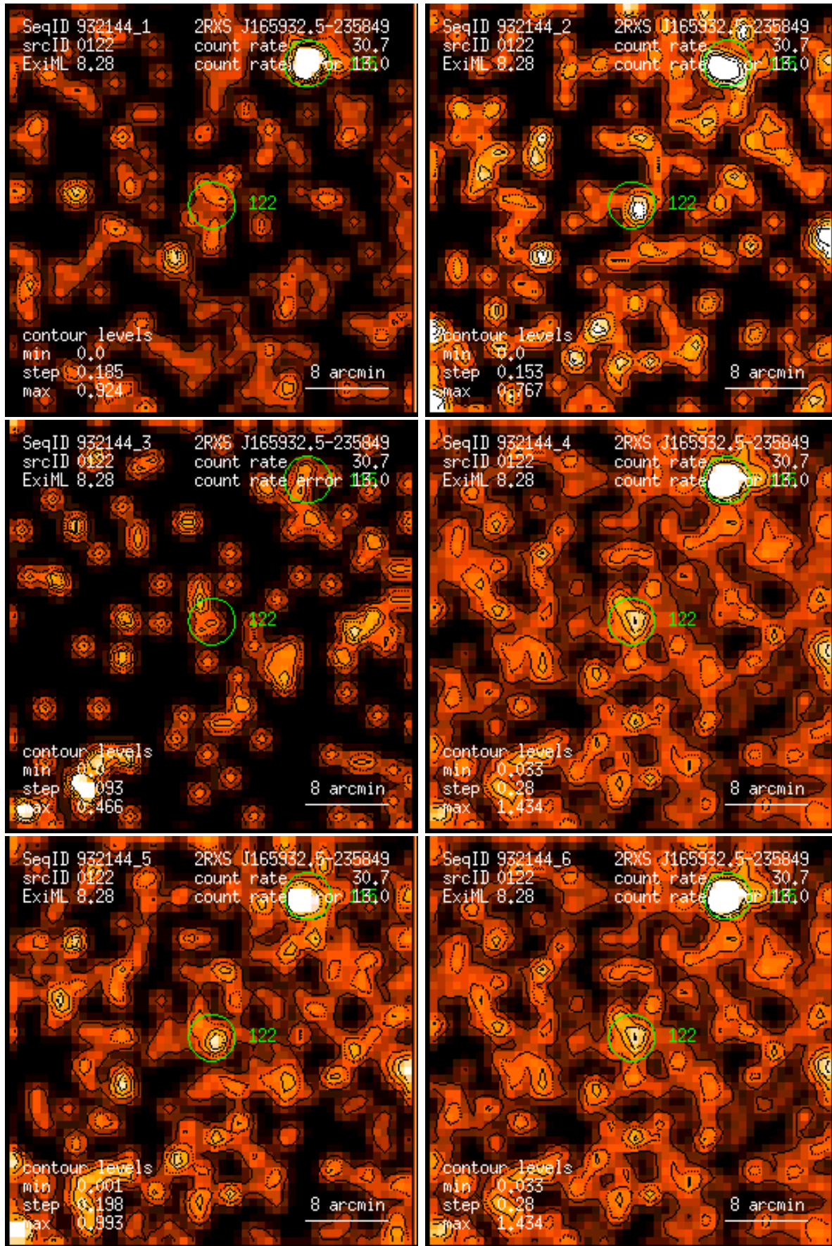
Figure 122: RASS 932144: detection 0122: band rate images, Gaussian filter: (1) PSPC channels 11 – 41, (2) 52 – 90, (3) 91 – 201, (4) 11 – 235, (5) 52 – 201, (6) 11 – 201. Broad band rates in counts/ks. Band rate contour levels in counts/ks/arcmin 2 .
