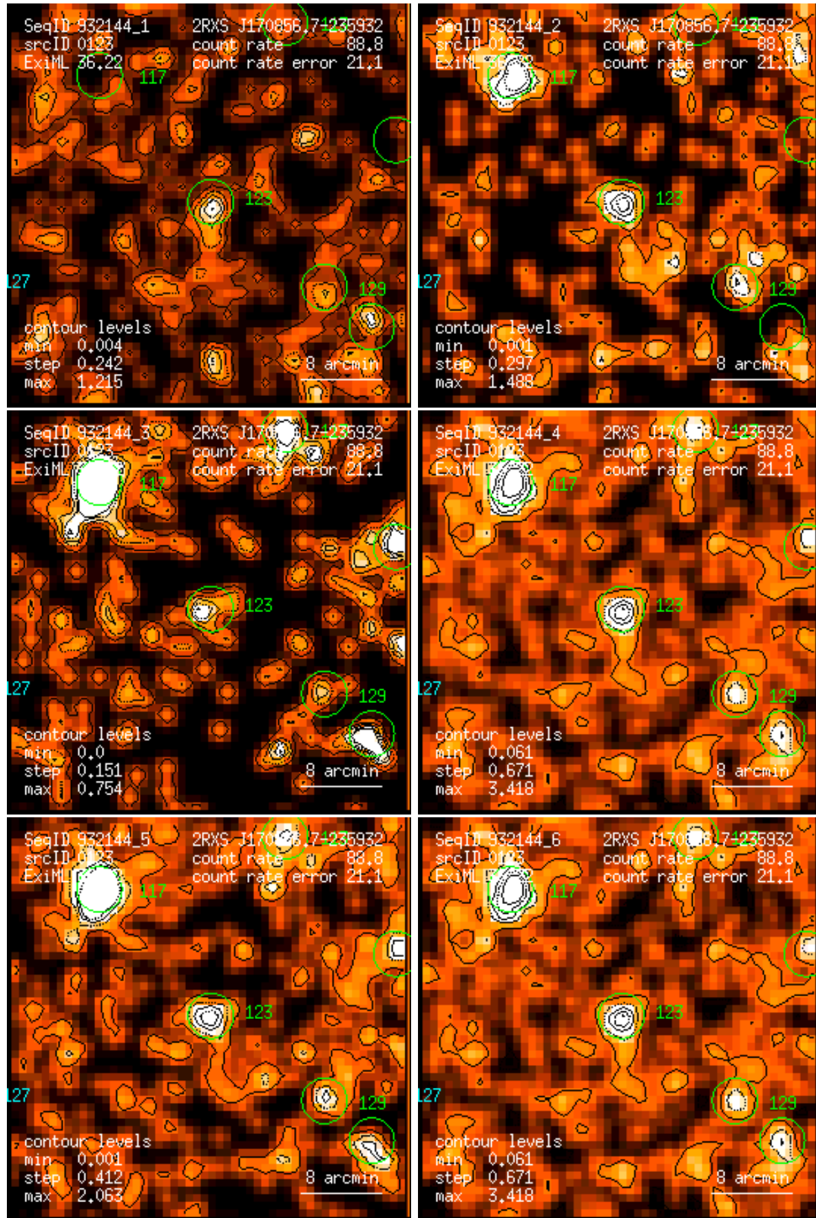
Figure 123: RASS 932144: detection 0123: band rate images, Gaussian filter: (1) PSPC channels 11 – 41, (2) 52 – 90, (3) 91 – 201, (4) 11 – 235, (5) 52 – 201, (6) 11 – 201. Broad band rates in counts/ks. Band rate contour levels in counts/ks/arcmin 2 .
