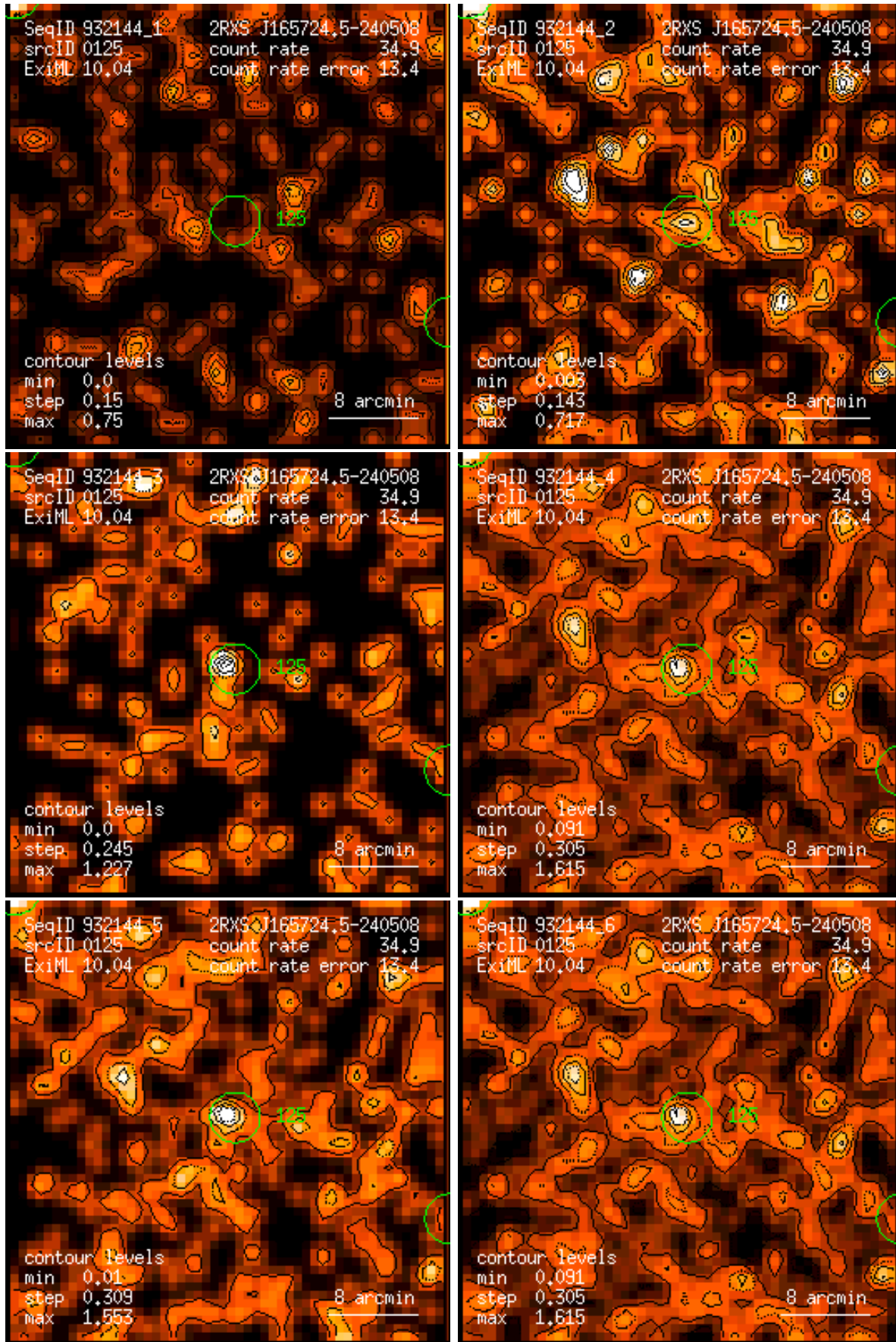
Figure 125: RASS 932144: detection 0125: band rate images, Gaussian filter: (1) PSPC channels 11 – 41, (2) 52 – 90, (3) 91 – 201, (4) 11 – 235, (5) 52 – 201, (6) 11 – 201. Broad band rates in counts/ks. Band rate contour levels in counts/ks/arcmin 2 .
