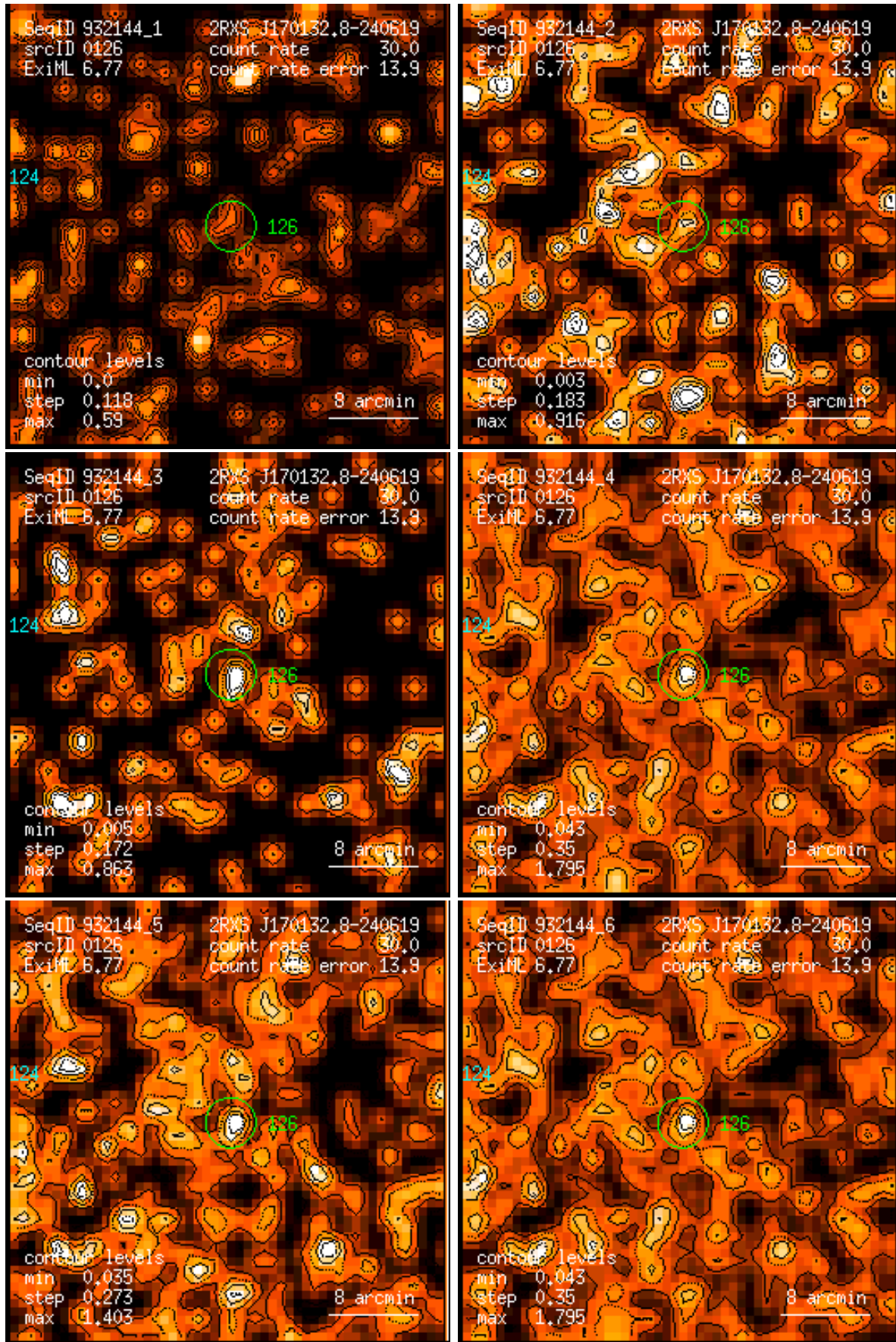
Figure 126: RASS 932144: detection 0126: band rate images, Gaussian filter: (1) PSPC channels 11 – 41, (2) 52 – 90, (3) 91 – 201, (4) 11 – 235, (5) 52 – 201, (6) 11 – 201. Broad band rates in counts/ks. Band rate contour levels in counts/ks/arcmin 2 .
