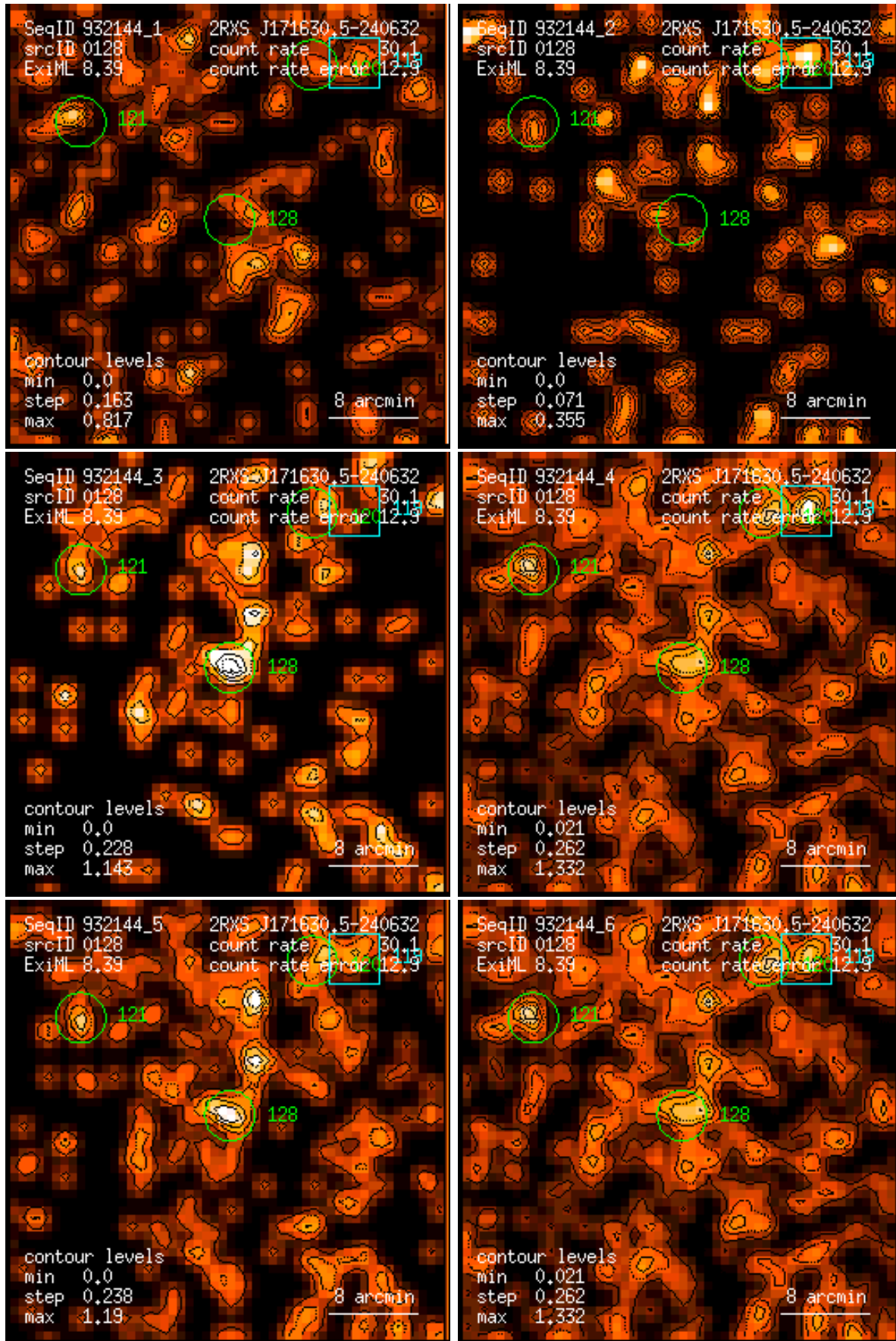
Figure 128: RASS 932144: detection 0128: band rate images, Gaussian filter: (1) PSPC channels 11 – 41, (2) 52 – 90, (3) 91 – 201, (4) 11 – 235, (5) 52 – 201, (6) 11 – 201. Broad band rates in counts/ks. Band rate contour levels in counts/ks/arcmin 2 .
