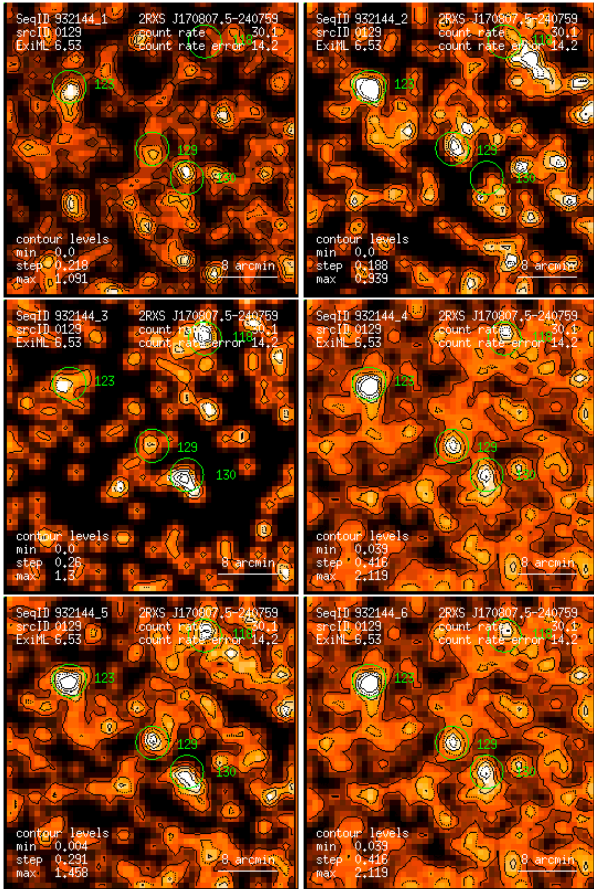
Figure 129: RASS 932144: detection 0129: band rate images, Gaussian filter: (1) PSPC channels 11 – 41, (2) 52 – 90, (3) 91 – 201, (4) 11 – 235, (5) 52 – 201, (6) 11 – 201. Broad band rates in counts/ks. Band rate contour levels in counts/ks/arcmin 2 .
