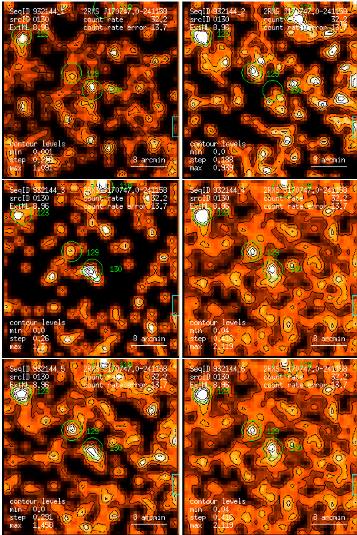
Figure 130: RASS 932144: detection 0130: band rate images, Gaussian filter: (1) PSPC channels 11 – 41, (2) 52 – 90, (3) 91 – 201, (4) 11 – 235, (5) 52 – 201, (6) 11 – 201. Broad band rates in counts/ks. Band rate contour levels in counts/ks/arcmin 2 .
