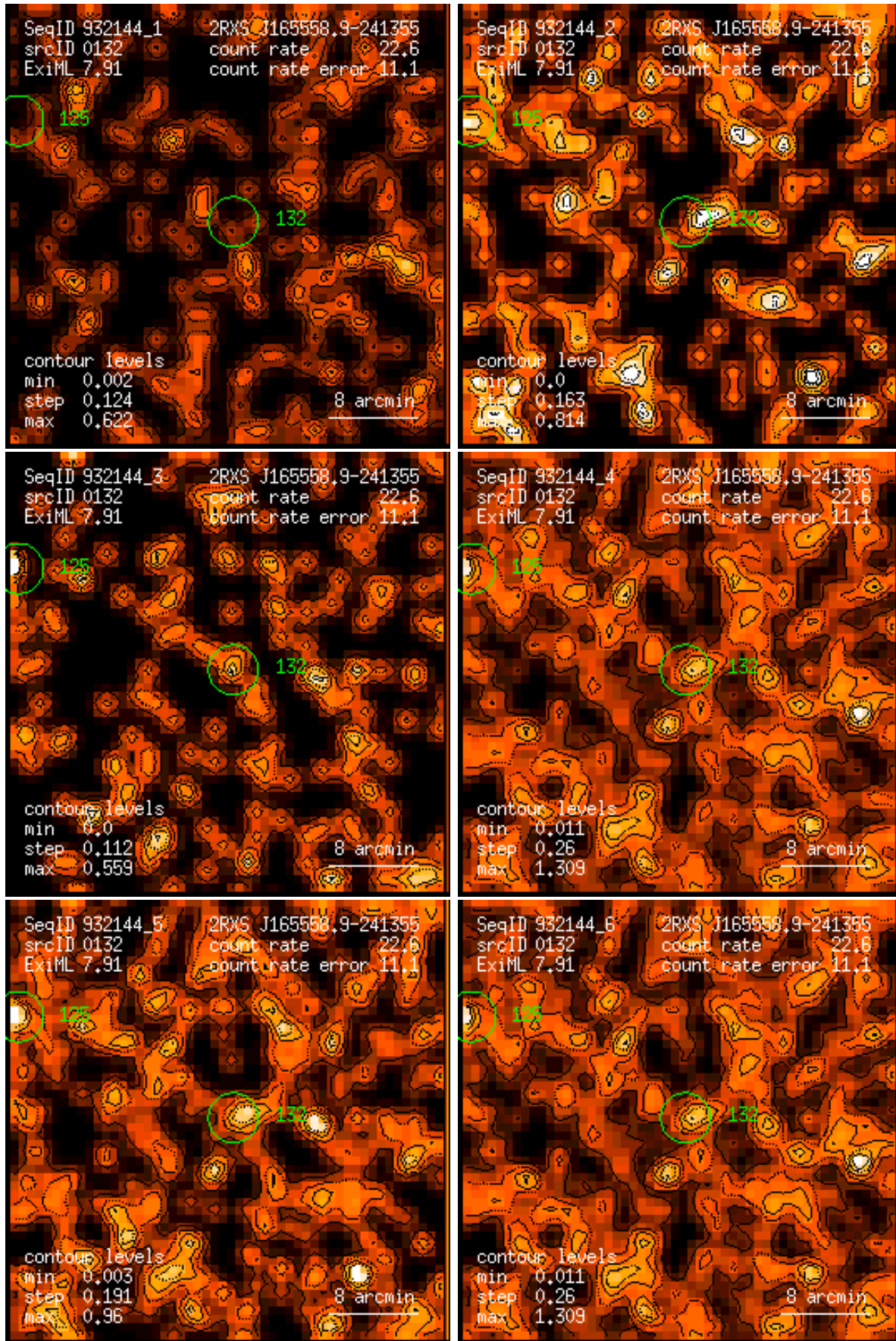
Figure 132: RASS 932144: detection 0132: band rate images, Gaussian filter: (1) PSPPC channels 11 – 41, (2) 52 – 90, (3) 91 – 201, (4) 11 – 235, (5) 52 – 201, (6) 11 – 201. Broad band rates in counts/ks. Band rate contour levels in counts/ks/arcmin 2 .
