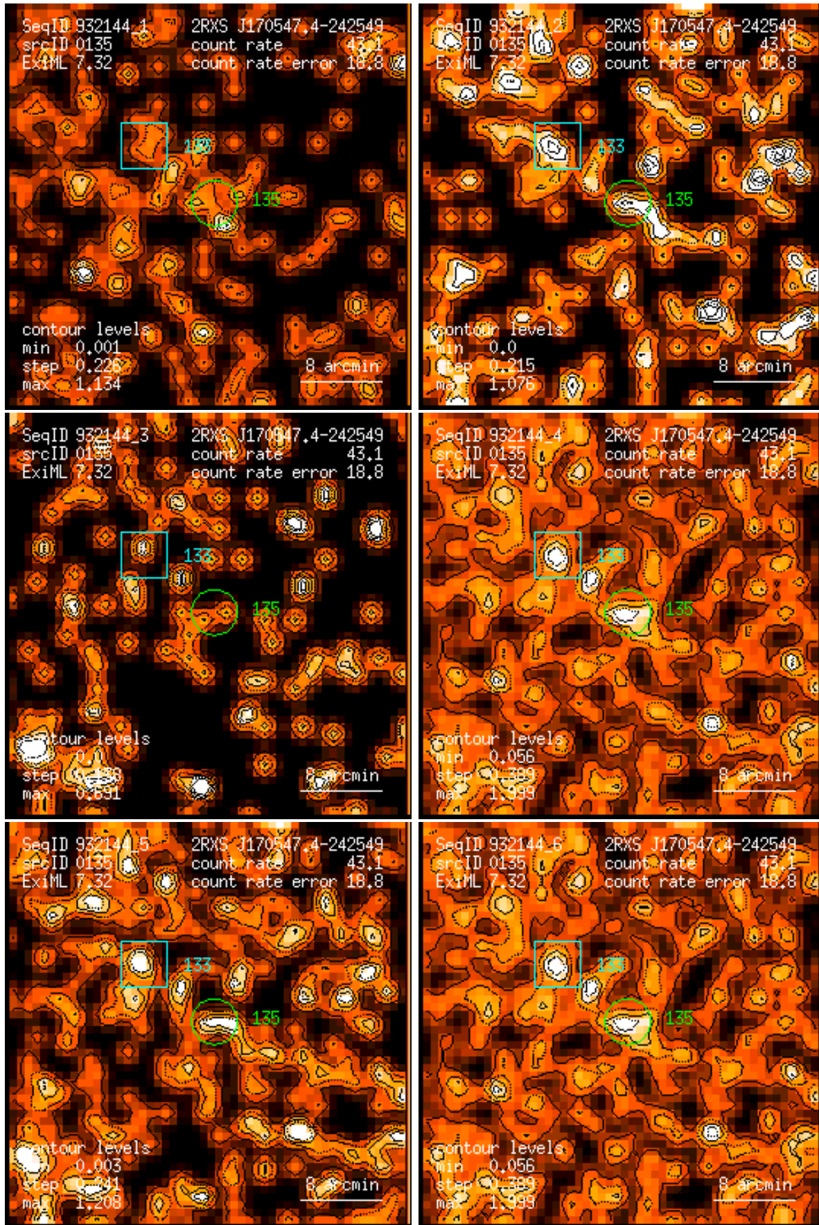
Figure 135: RASS 932144: detection 0135: band rate images, Gaussian filter: (1) PSPC channels 11 – 41, (2) 52 – 90, (3) 91 – 201, (4) 11 – 235, (5) 52 – 201, (6) 11 – 201. Broad band rates in counts/ks. Band rate contour levels in counts/ks/arcmin 2 .
