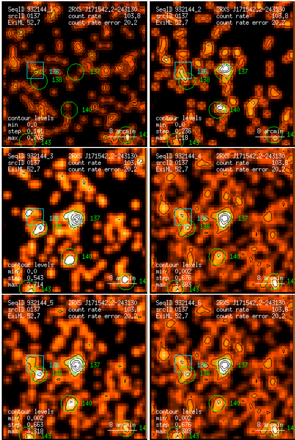
Figure 137: RASS 932144: detection 0137: band rate images, Gaussian filter: (1) PSPC channels 11 – 41, (2) 52 – 90, (3) 91 – 201, (4) 11 – 235, (5) 52 – 201, (6) 11 – 201. Broad band rates in counts/ks. Band rate contour levels in counts/ks/arcmin 2 .
