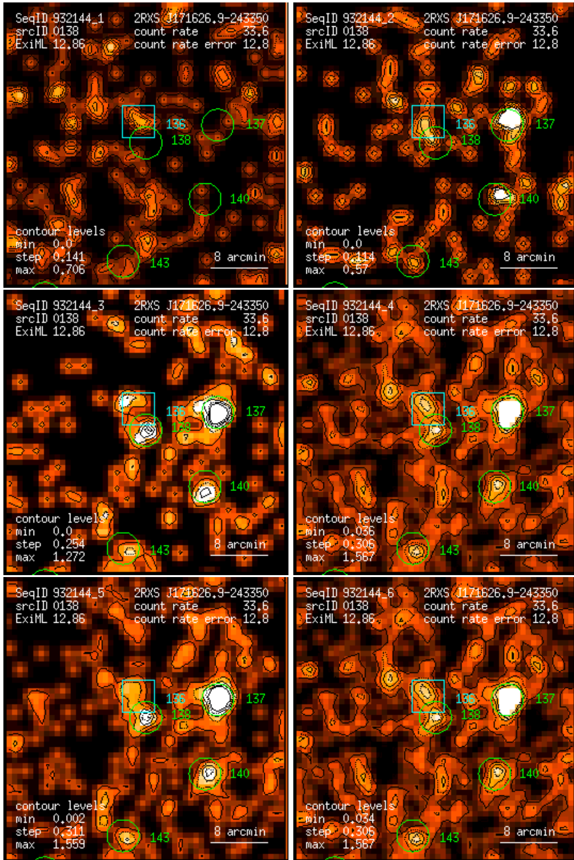
Figure 138: RASS 932144: detection 0138: band rate images, Gaussian filter: (1) PSPC channels 11 – 41, (2) 52 – 90, (3) 91 – 201, (4) 11 – 235, (5) 52 – 201, (6) 11 – 201. Broad band rates in counts/ks. Band rate contour levels in counts/ks/arcmin 2 .
