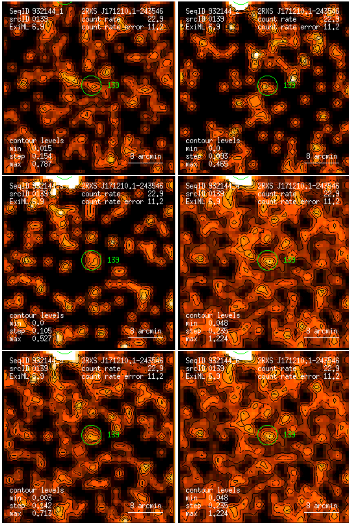
Figure 139: RASS 932144: detection 0139: band rate images, Gaussian filter: (1) PSPC channels 11 – 41, (2) 52 – 90, (3) 91 – 201, (4) 11 – 235, (5) 52 – 201, (6) 11 – 201. Broad band rates in counts/ks. Band rate contour levels in counts/ks/arcmin 2 .
