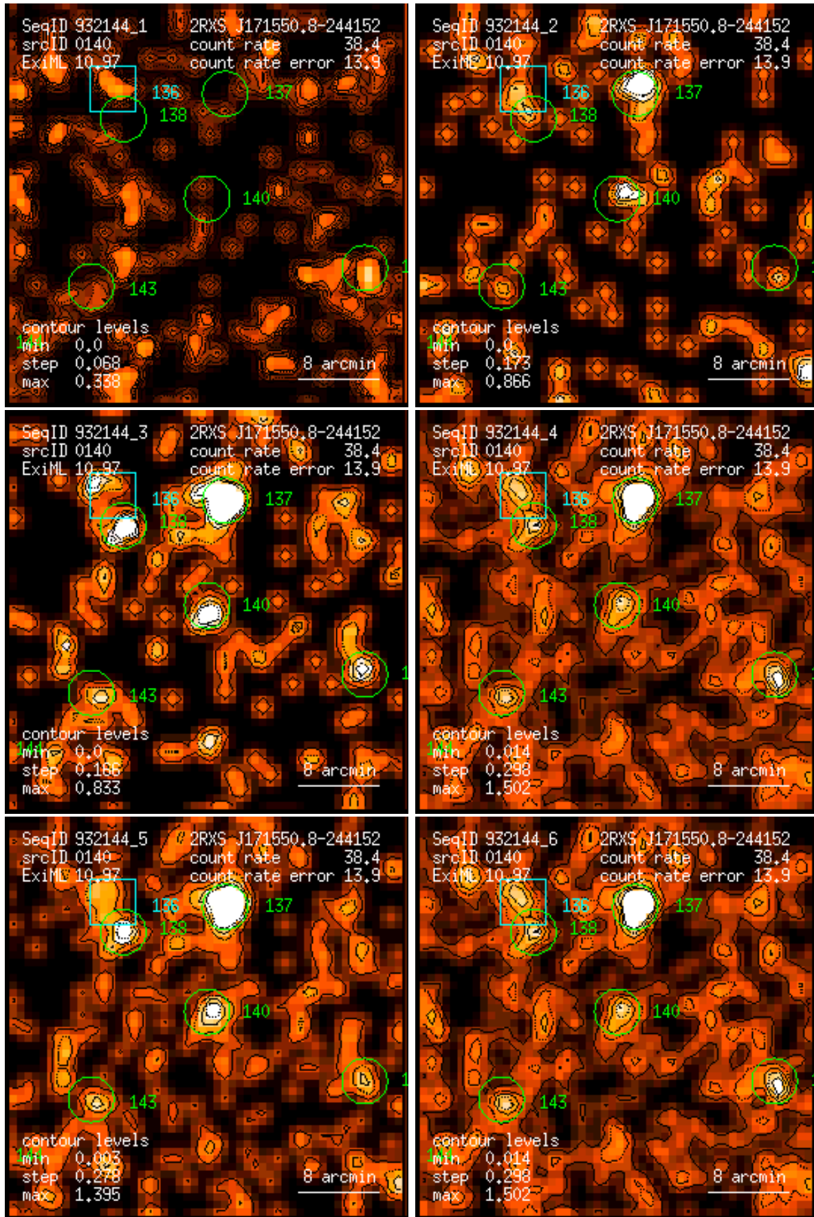
Figure 140: RASS 932144: detection 0140: band rate images, Gaussian filter: (1) PSPC channels 11 – 41, (2) 52 – 90, (3) 91 – 201, (4) 11 – 235, (5) 52 – 201, (6) 11 – 201. Broad band rates in counts/ks. Band rate contour levels in counts/ks/arcmin 2 .
